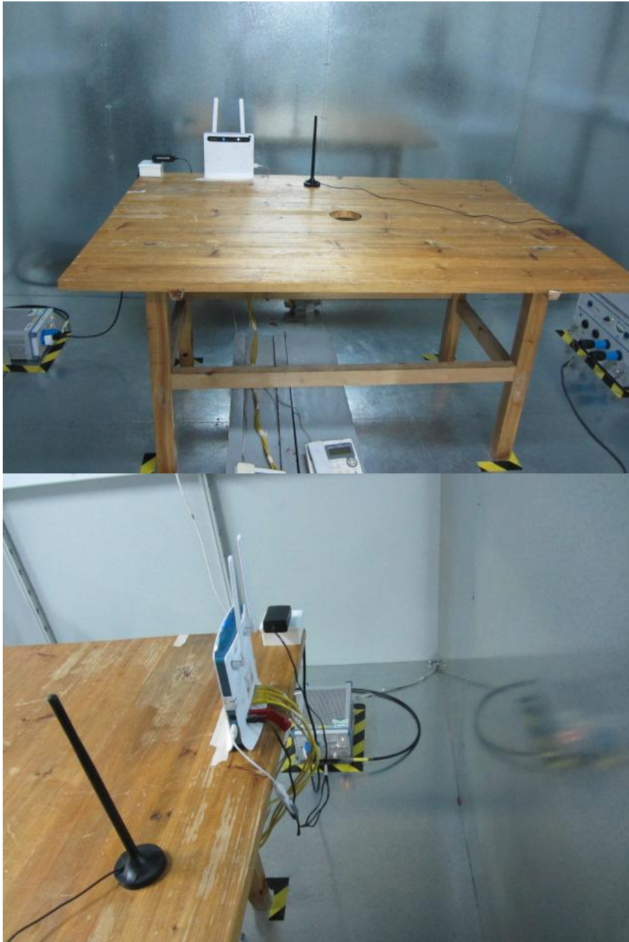
Conducted Emissions for AC Ports
