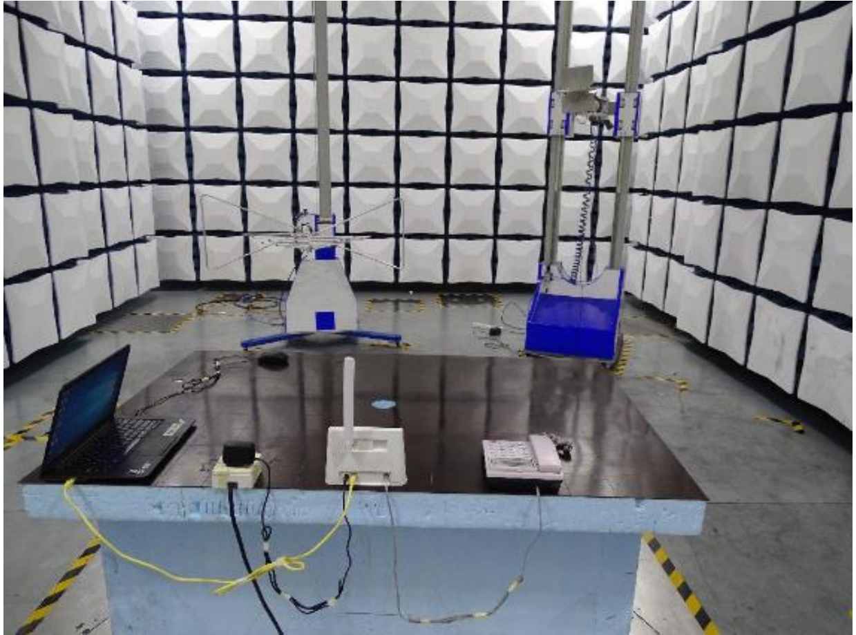
Radiated Disturbance Emissions (below 1GHz)
