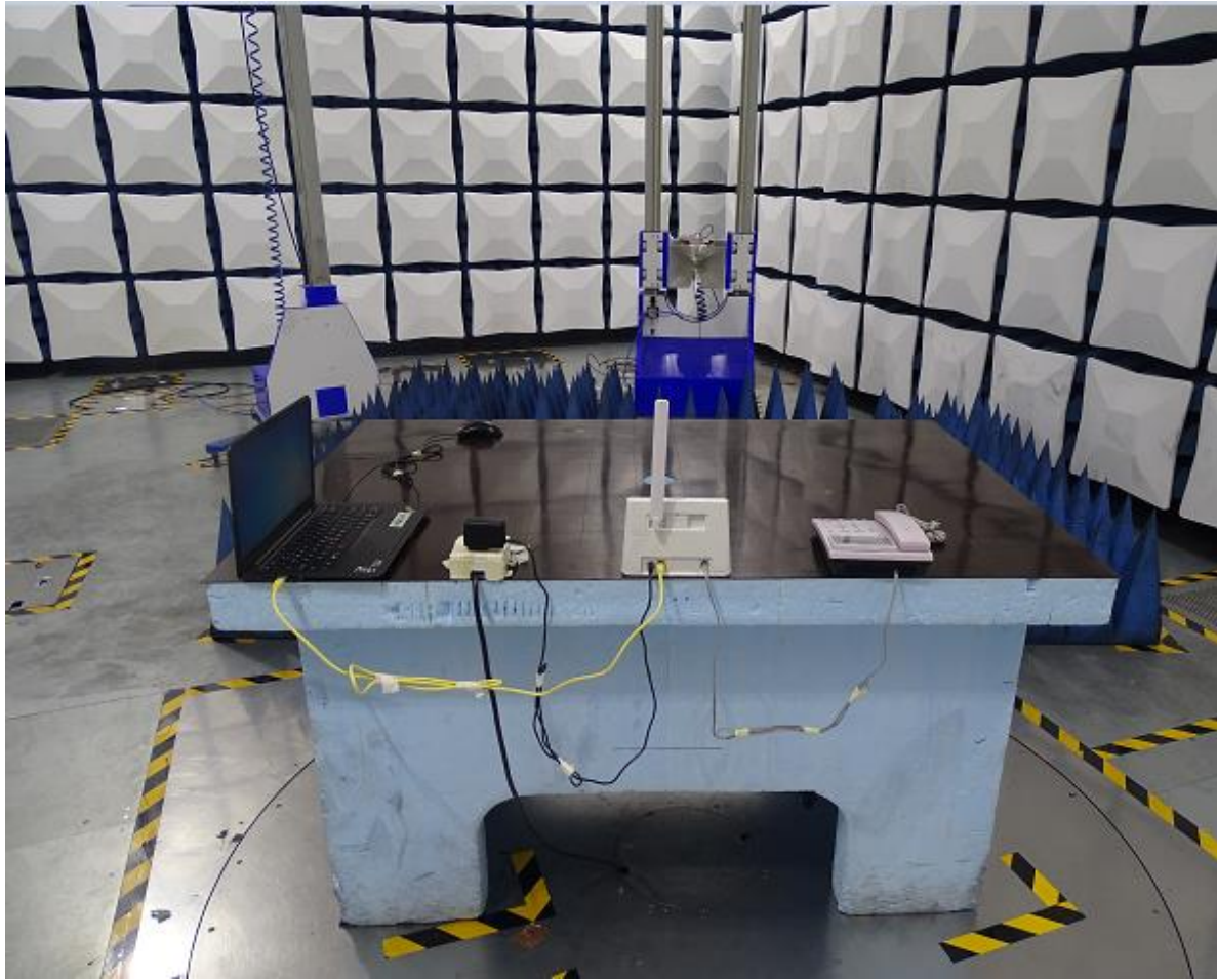
Radiated Disturbance Emissions (1GHz to18GHz)
