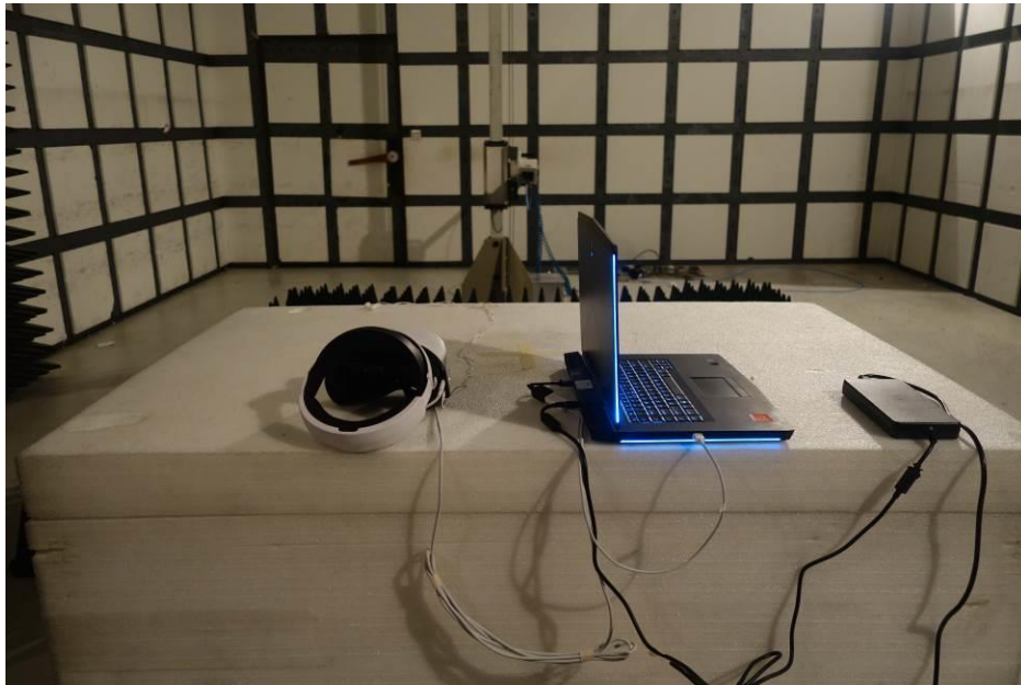
Radiated Disturbance Emissions (18GHz to 26.5GHz)
