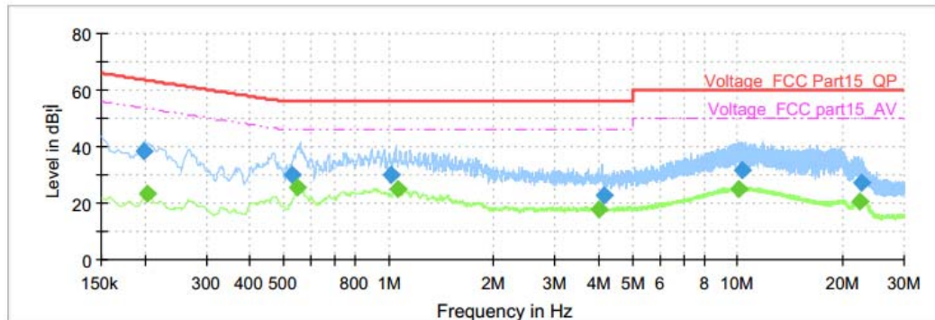
BT_L_0.15-30Mhz
