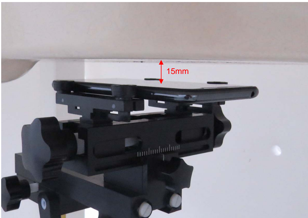
Picture 6: Front Side, the distance from handset to the bottom of the Phantom is 15mm (ATU-L11)
