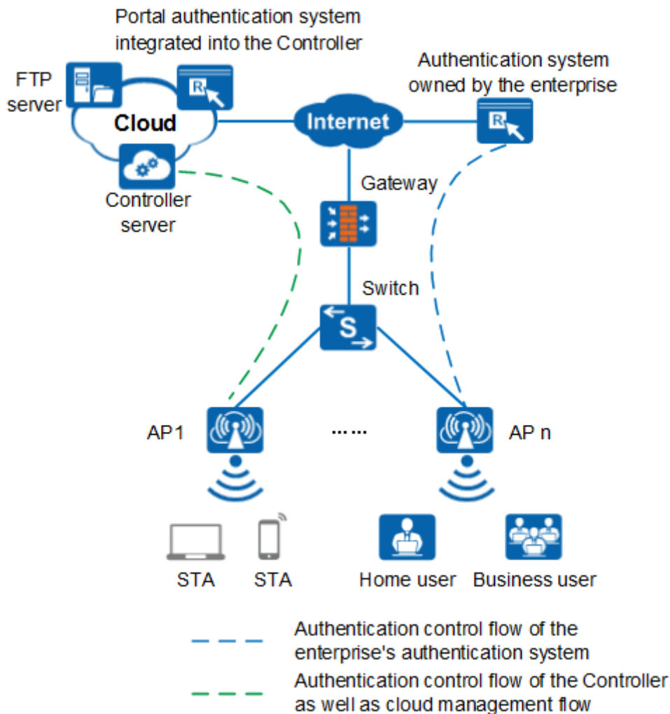
Figure 1-3 Cloud AP networking
