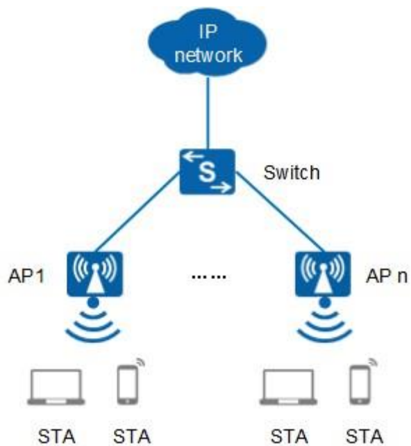
Figure 1-2 Fat AP networking
