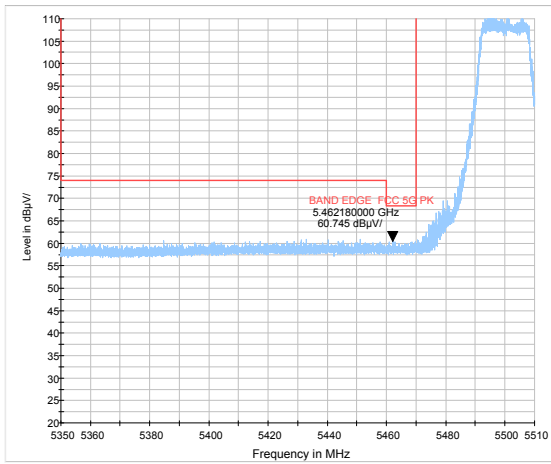
802.11a-Channel 100: Peak
