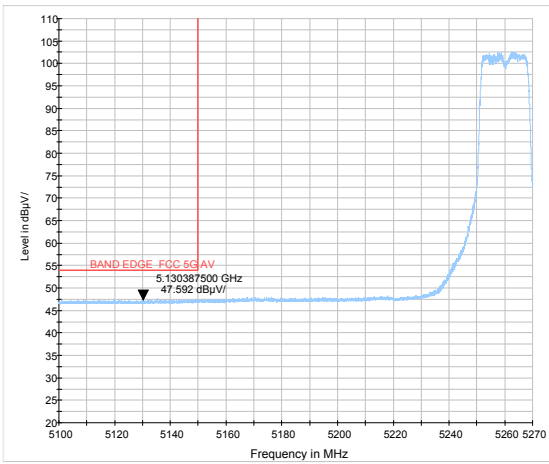
802.11a-Channel 52: Average
