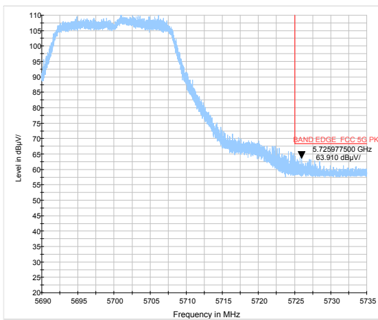
802.11a-Channel 140: Peak
