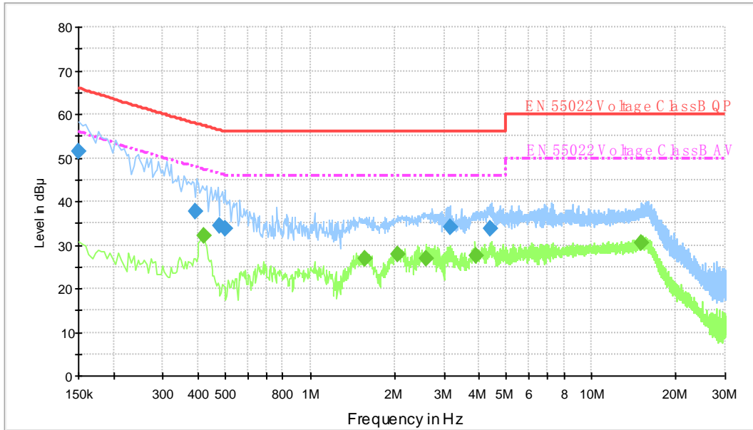
Voltage with 4-Line-LISN
