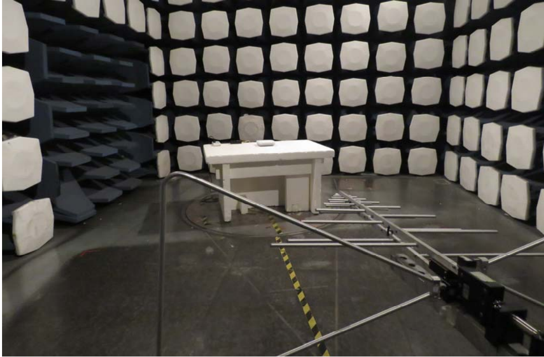
FCC Part15E Radiated Emission Test Setup
