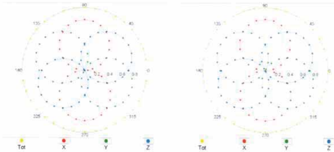
f=600 MHz,TEM
