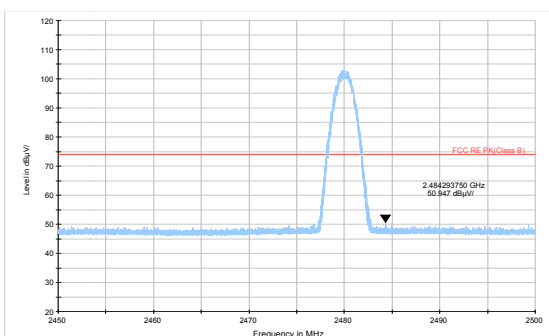
3DH5-Channel 78: Peak
