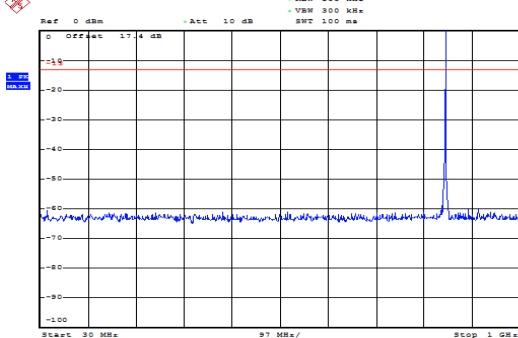
GSM 850 CH-High 30MHz ~ 1GHz
