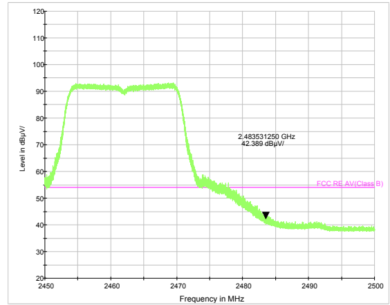
802.11g-Channel 11 Average
