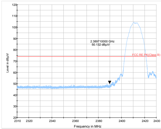
802.11b-Channel 1 Peak
