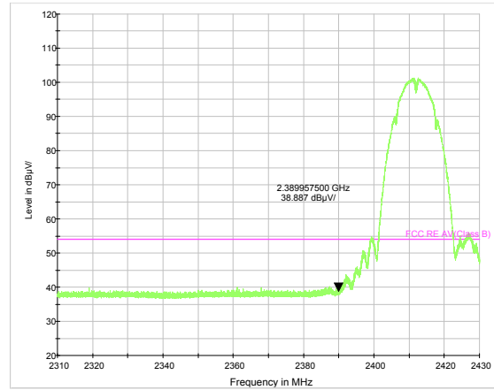
802.11b-Channel 1 Average
