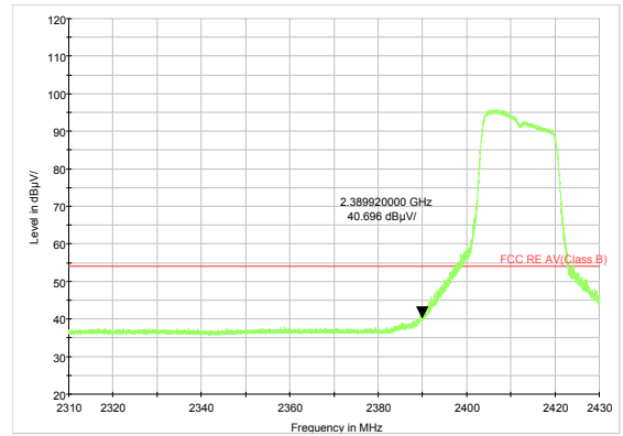
802.11g-Channel 1 Average
