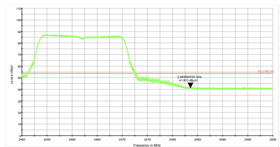
802.11g-Channel 11 Average
