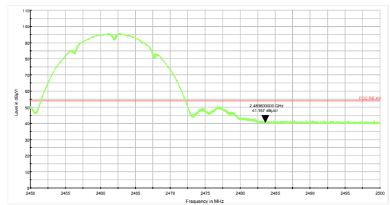
802.11b-Channel 11 Average
