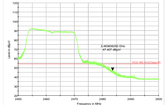
802.11g-Channel 11 Average
