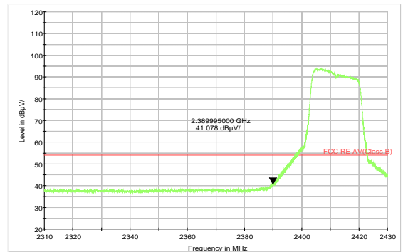
802.11g-Channel 1 Average
