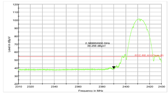
802.11b-Channel 1 Average
