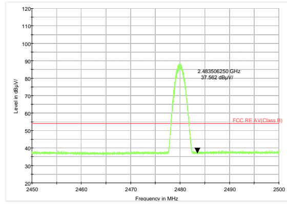
BLE V 5.0 Channel 39 Average
