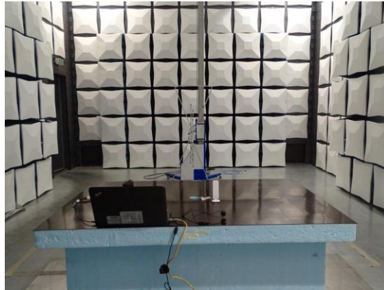
Radiated Spurious Emission (below 3GHz)
