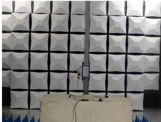
Radiated Spurious Emission (above 18GHz)
