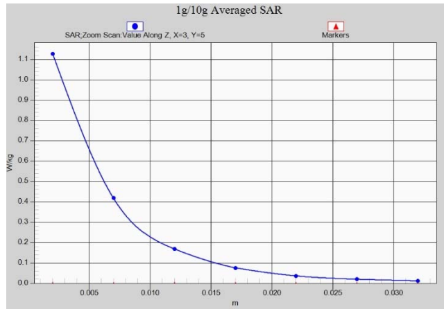
Fig.A.1- 7 Z-Scan at power reference point (WiFi 2.4G)
