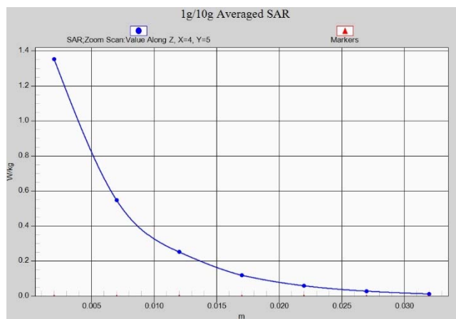
Fig.A.1- 6 Z-Scan at power reference point (LTE band 7)
