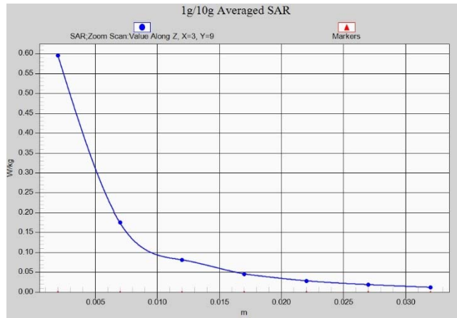
Fig.A.1- 4 Z-Scan at power reference point (W850)
