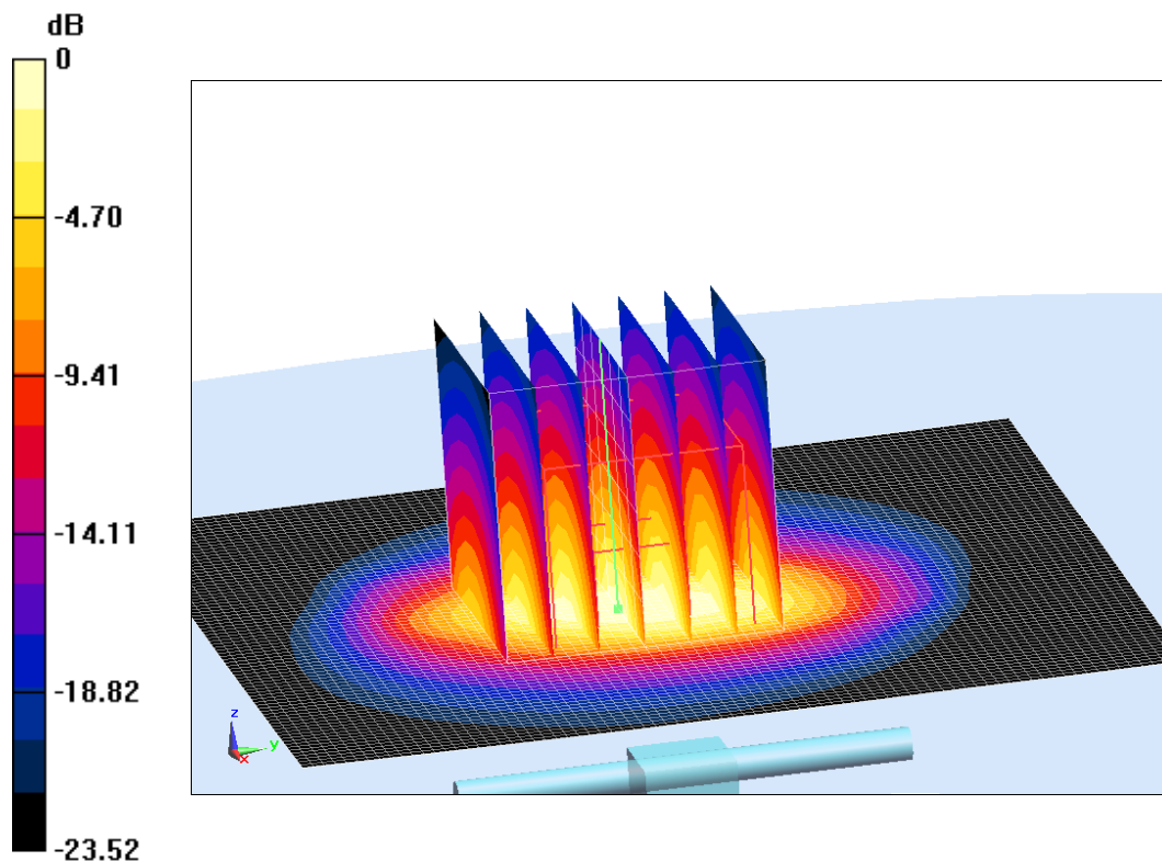
Fig.B.3 validation 2600 MHz 250mW
