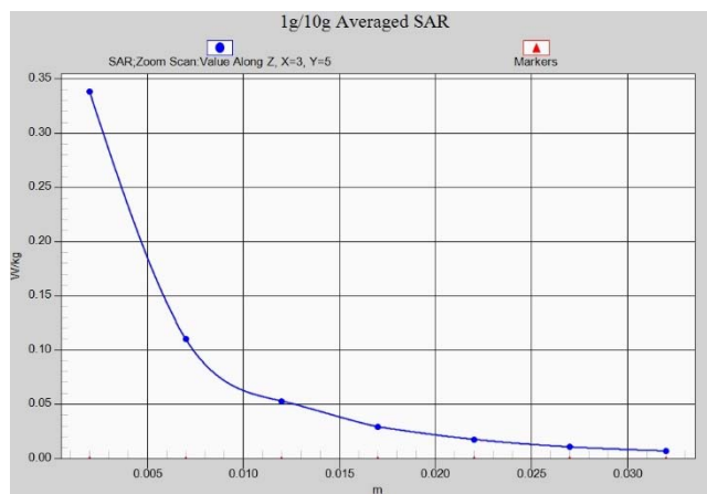
Fig.A.1- 5 Z-Scan at power reference point (LTE band 5)
