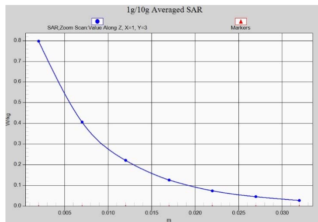
Fig.A.1- 3 Z-Scan at power reference point (W1900)
