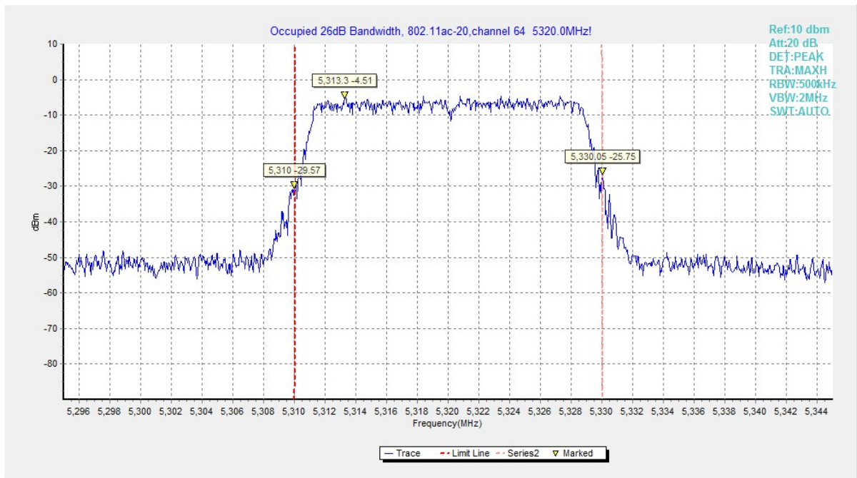
Fig. 24 Occupied 26dB Bandwidth (802.11ac20, 5320MHz)
