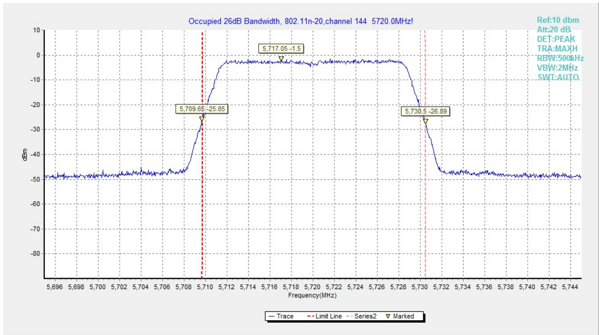
Fig. 18 Occupied 26dB Bandwidth (802.11n20, 5720MHz)
