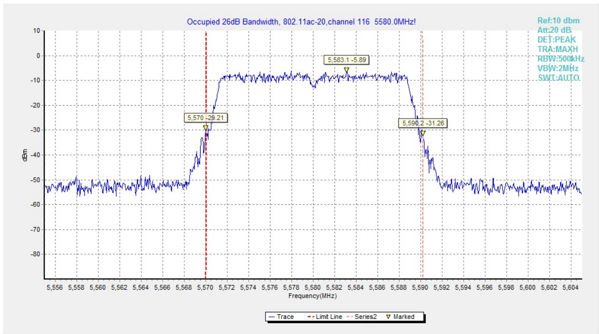
Fig. 26 Occupied 26dB Bandwidth (802.11ac20, 5580MHz)
