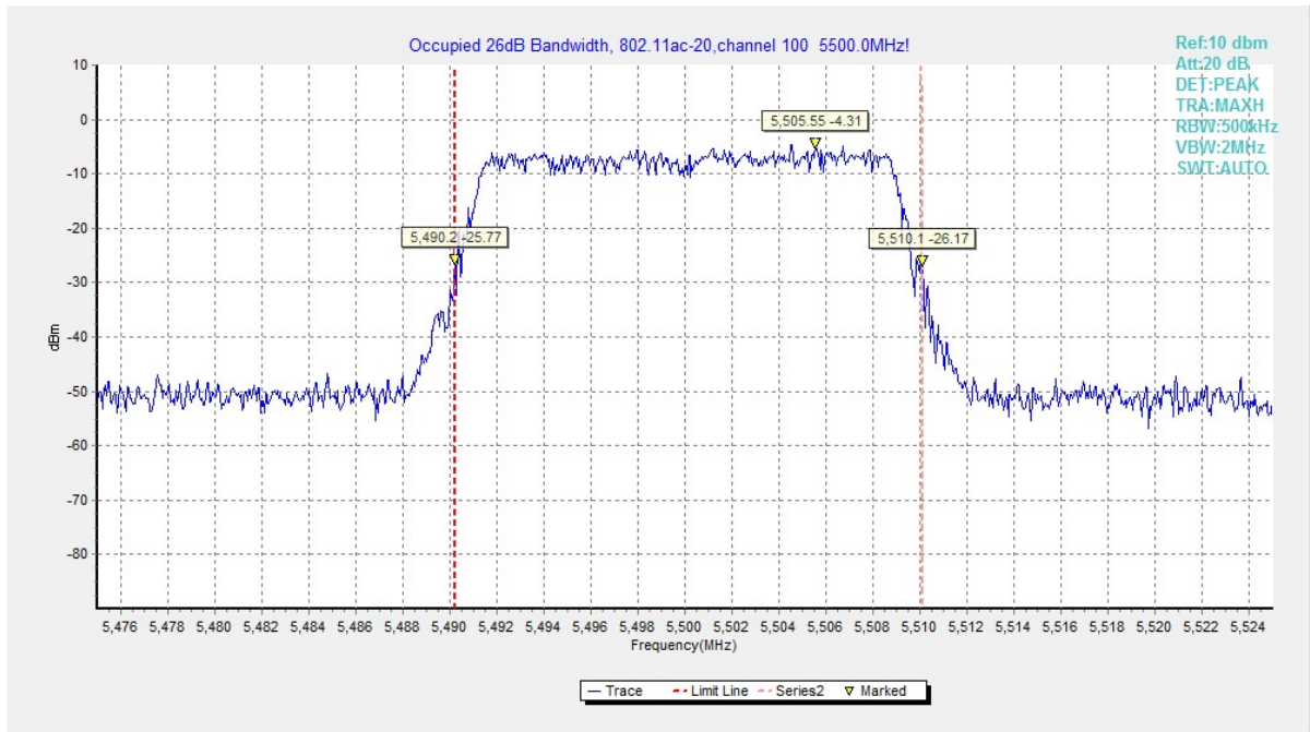
Fig. 25 Occupied 26dB Bandwidth (802.11ac20, 5500MHz)
