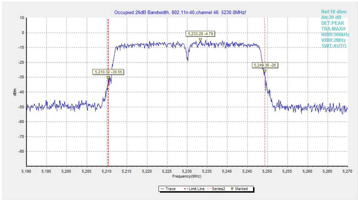
Fig. 29 Occupied 26dB Bandwidth (802.11n40, 5230MHz)
