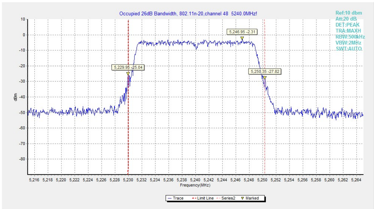
Fig. 12 Occupied 26dB Bandwidth (802.11n20, 5240MHz)
