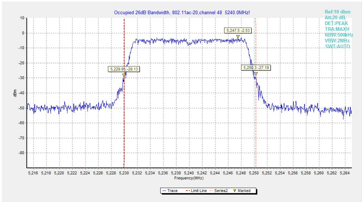
Fig. 21 Occupied 26dB Bandwidth (802.11ac20, 5240MHz)
