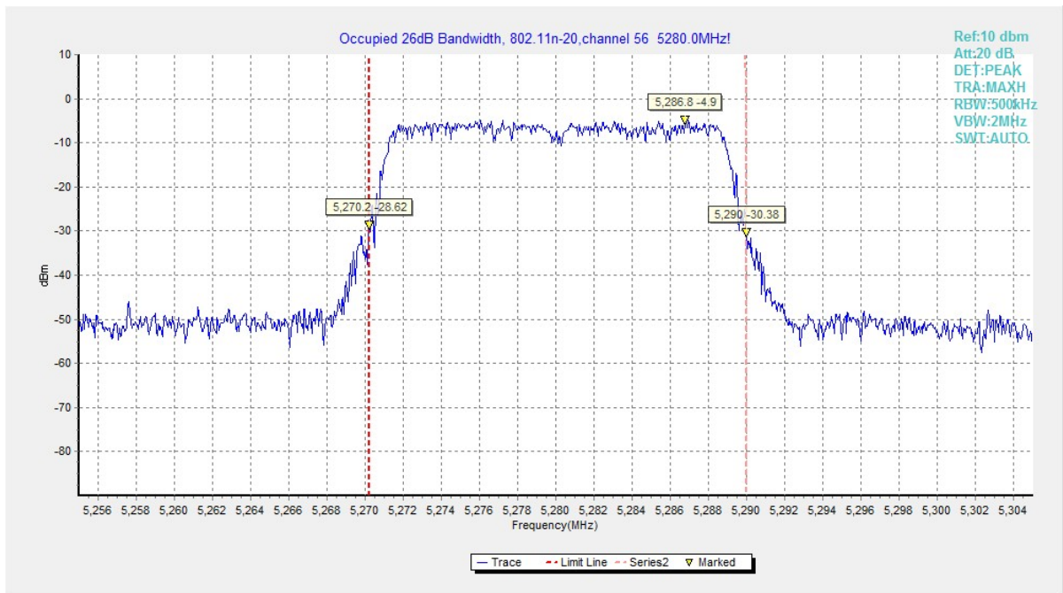
Fig. 14 Occupied 26dB Bandwidth (802.11n20, 5280MHz)
