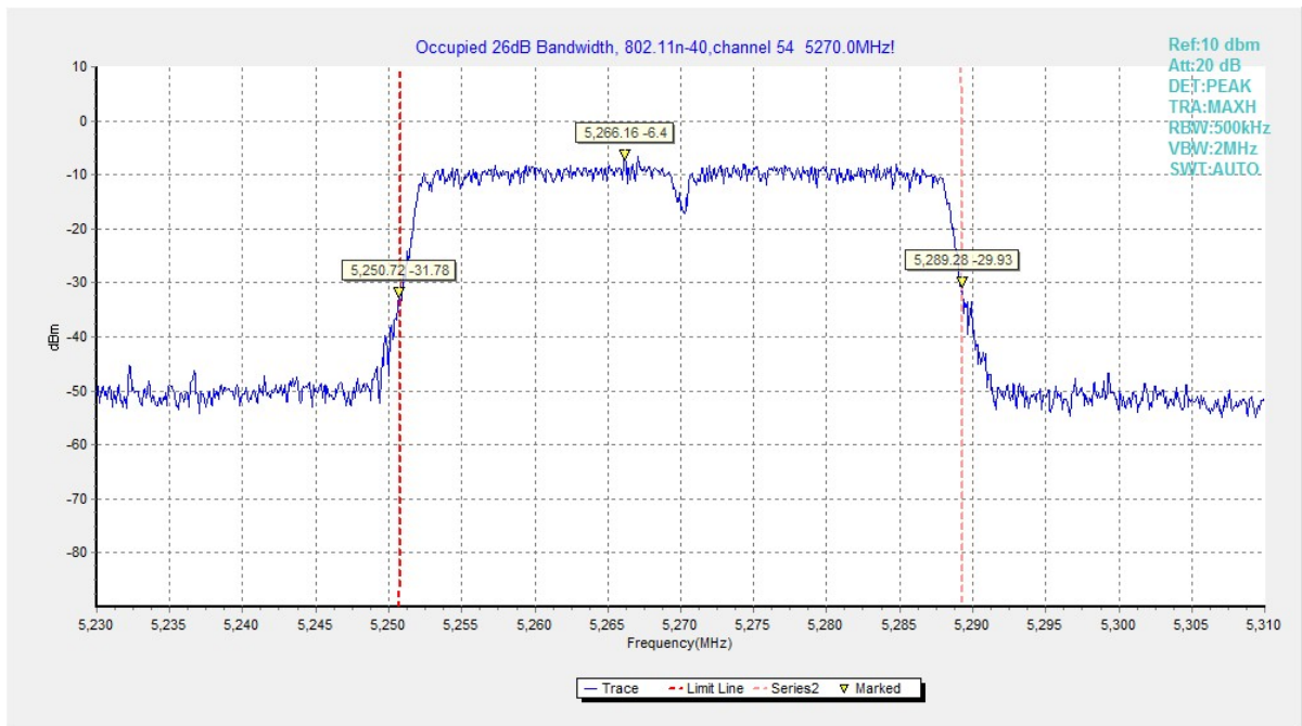
Fig. 30 Occupied 26dB Bandwidth (802.11n40, 5270MHz)
