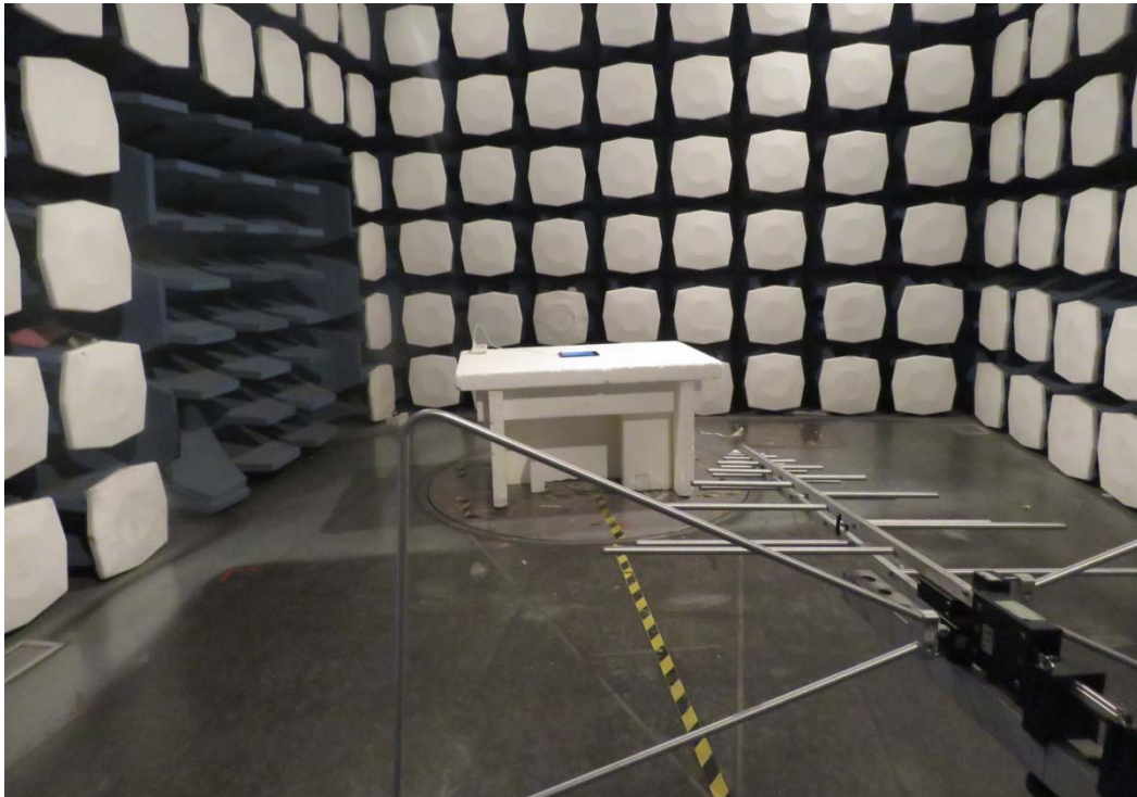
30M Hz-1GHz
