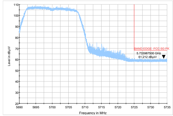
802.11a-Channel 140: Peak
