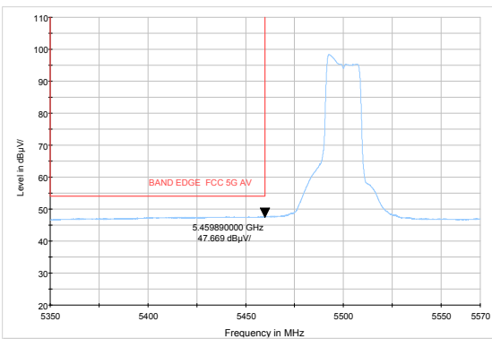
802.11a-Channel 100: Average
