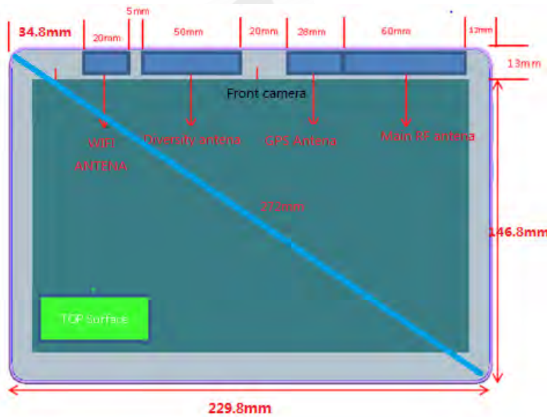
Fig.10 Antenna position of EUT (Front view)
