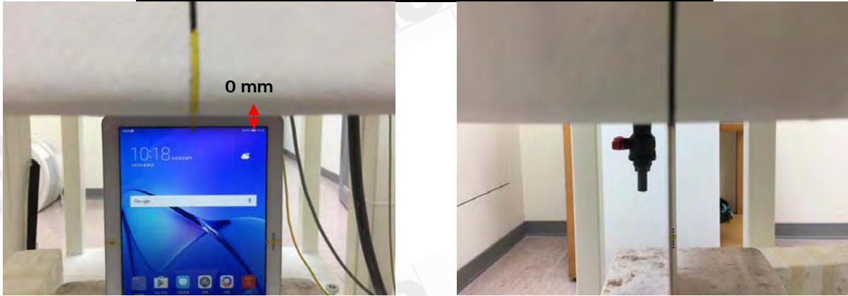
Fig.6 EUT Right side to flat phantom
