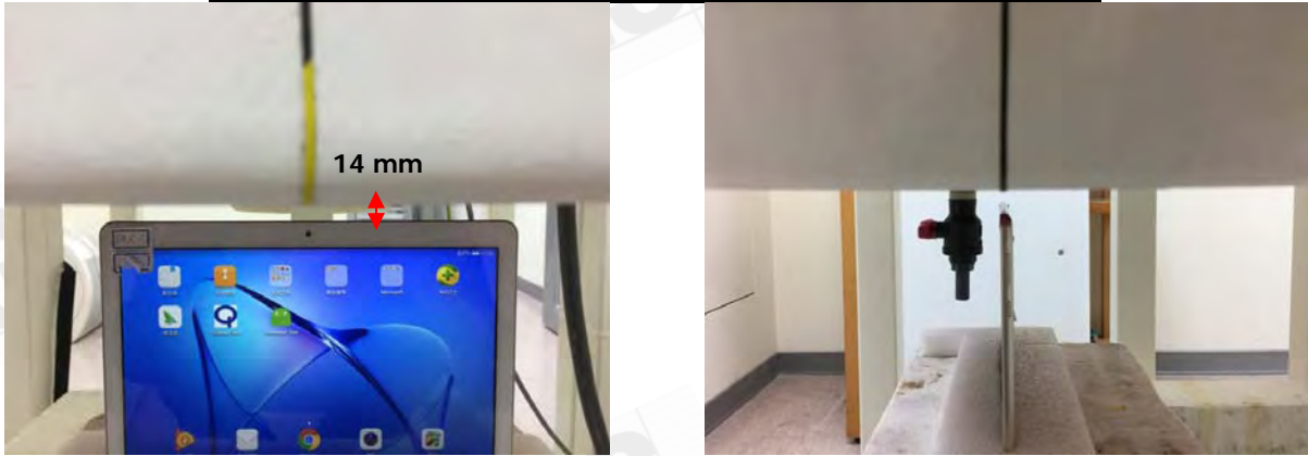
Fig.9 EUT Top side (14mm) to flat phantom
