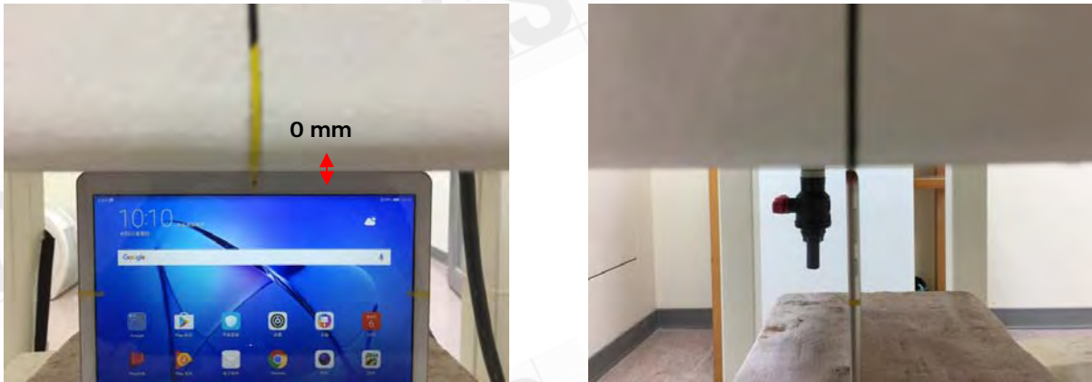
Fig.7 EUT Top side to flat phantom
