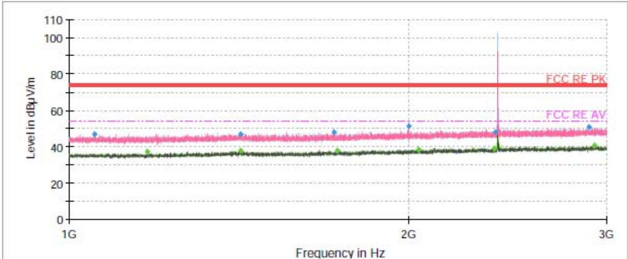
Note: The signal beyond the limit is carrier. Radiates Emission from 1GHz to 3GHz
