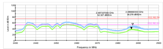
802.11n HT40 -Channel 9 Peak+ Average
