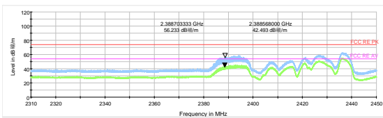
802.11n HT40 -Channel 3 Peak+ Average
