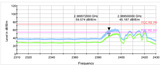
802.11n HT20 -Channel 1 Peak+ Average
