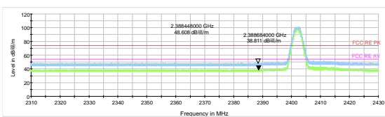
Bluetooth LE (2M) Channel 0 Peak+ Average
