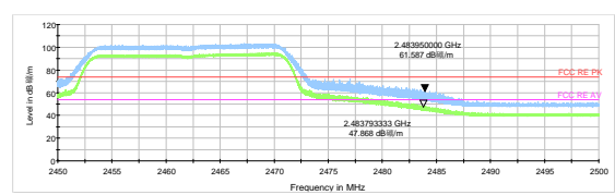
802.11n HT20 -Channel 11 Peak+ Average
