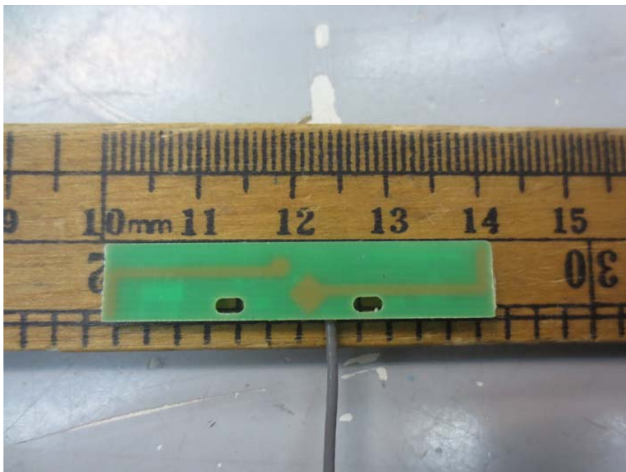
Internal Antenna (Ant 3)
