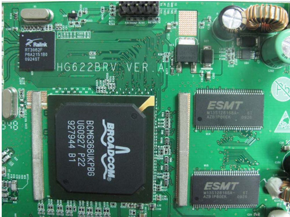
(4) EUT Photo (HG622)
