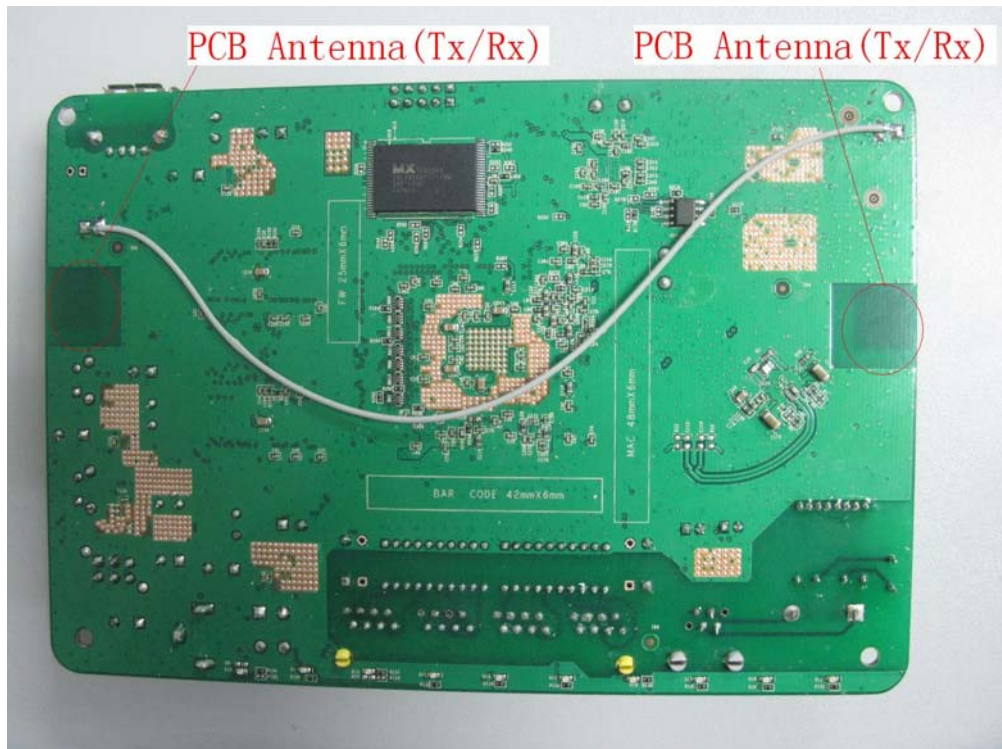
(2) EUT Photo (HG622)
