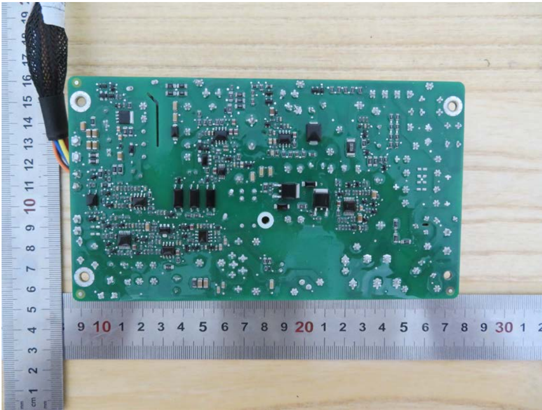
Power Supply(Manufacturer : ASTEC)
