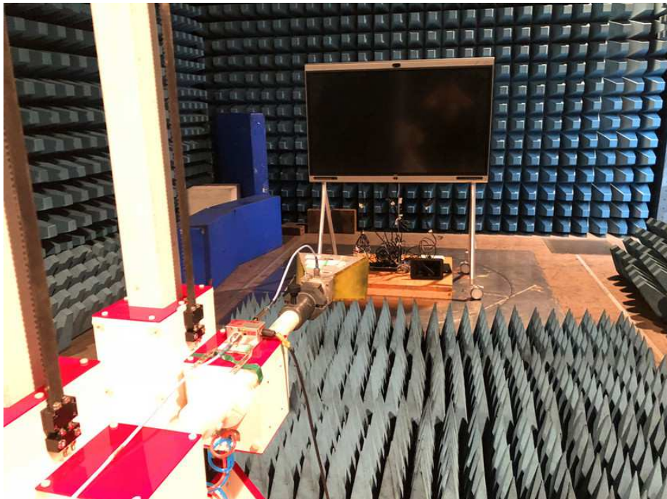
Above 1GHz
