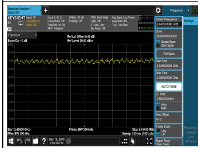
8DPSK, Hopping, 3DH5, 2426.5~2454.5MHz
