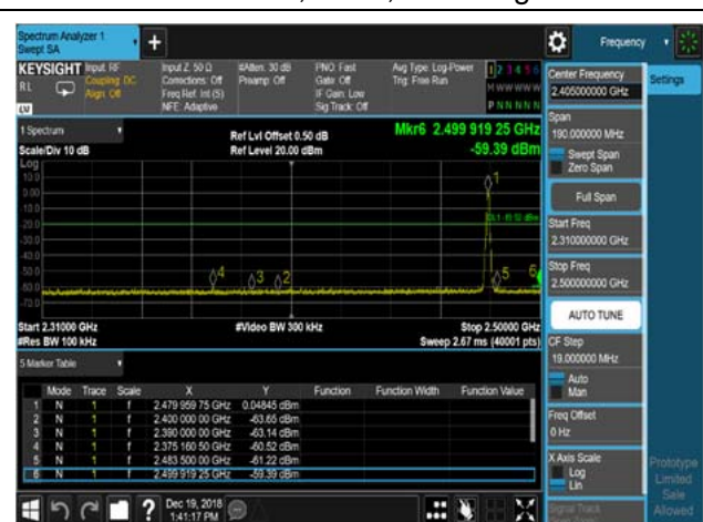
2480MHz, Plot 2, Band Edge
