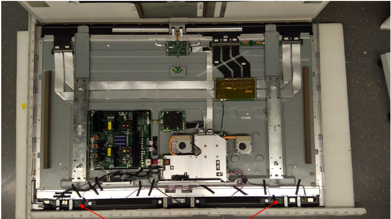
RF Antenna
