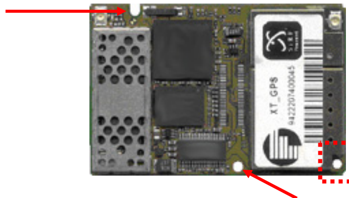
Figure 52: Mounting holes on XT55/56
