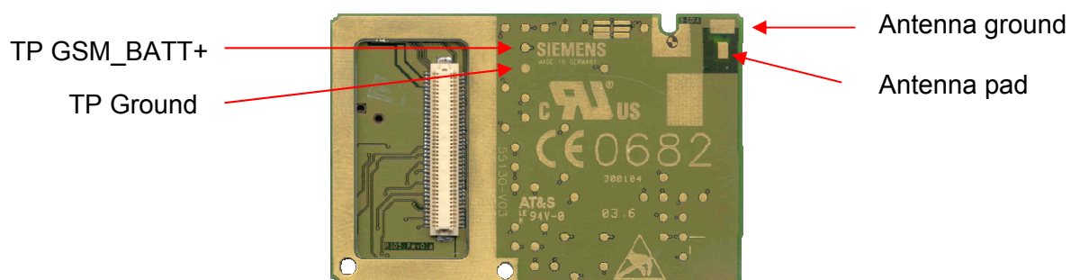
Figure 50: XT55/56 bottom view
