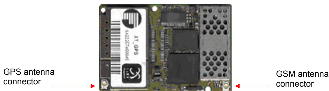
Figure 49: XT55/56 – top view
