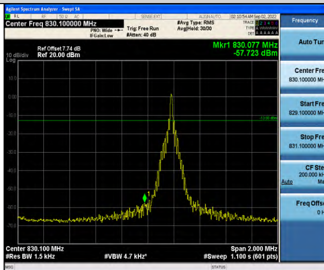
Band19-Stand-Alone-Na-N-BPSK-24002-1 @ 11-15kHz--57.72-PASS
