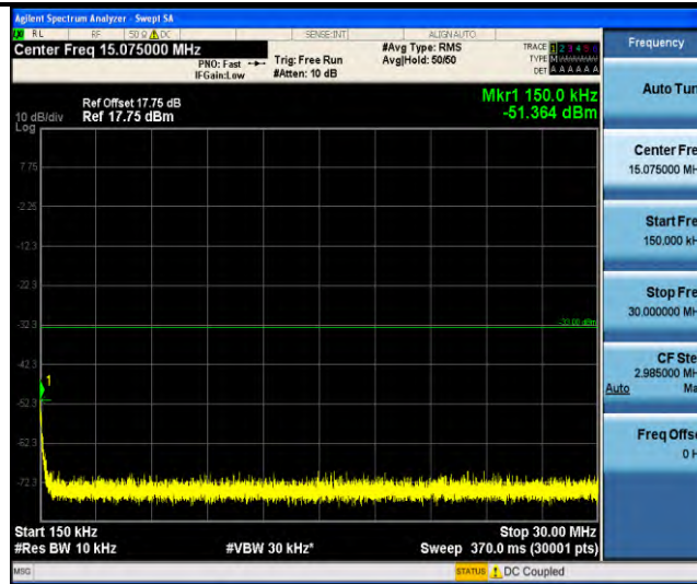
Band66-Stand-Alone-Na-N-QPSK-132322-1 @ 47-3.75kHz-0.15-30-0.15~30MHz @ -51.36dBm--33-PASS
