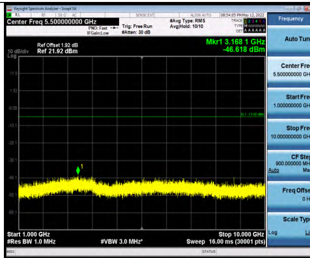
Band26-Stand-Alone-NaN-BPSK-26740-1 @ 11-15kHz-1000-10000-1000~10000MHz @ -46.62dBm--13-PASS
