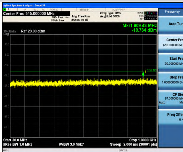
Band66-Stand-Alone-NaN-BPSK-132322-1 @ 11-15kHz-30-1000-30~1000MHz @ -18.73dBm--13-PASS
