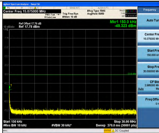
Band25-Stand-Alone-NaN-QPSK-26365-1 @ 47-3.75kHz-0.15-30-0.15~30MHz@ -49.32dBm--33-PASS
