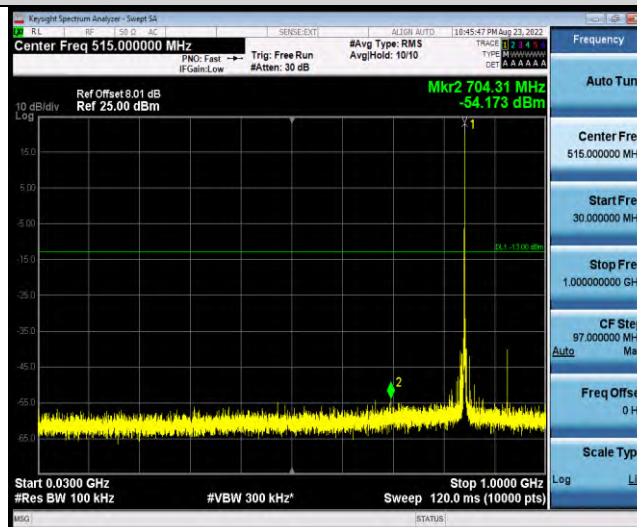
Band19-Stand-Alone-Na-N-QPSK-24148-12@0-15kHz-30-1000-30~1000MHz@-54.17dBm--13-PASS
