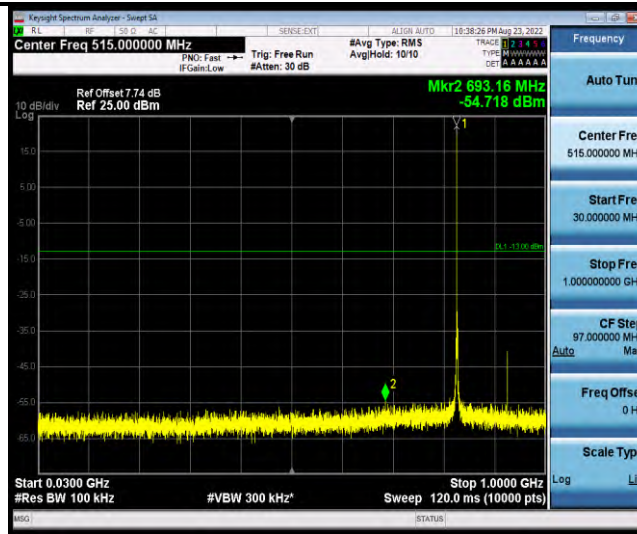
Band19-Stand-Alone-NaN-QPSK-24002-1 @0-3.75kHz-30-1000-30~1000MHz@-54.72dBm--13-PASS
