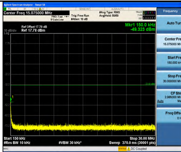
Band25-Stand-Alone-NaN-QPSK-26365-1 @ 47-3.75kHz-0.15-30-0.15~30MHz @ -49.32dBm--33-PASS
