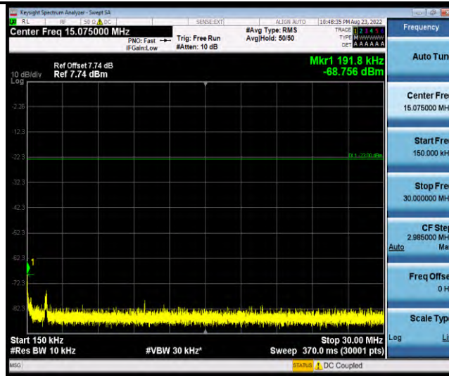
Band19-Stand-Alone-NaN-BPSK-24002-1 @ 11-15kHz-0.15-30-0.15~30MHz @ -68.76dBm--23-PASS
