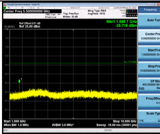
Band19-Stand-Alone-NaN-QPSK-24148-12@0-15kHz-1000-10000-1000~10000MHz@-35.72dBm--13-PASS
