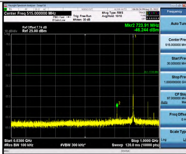
Band18-Stand-Alone-NaN-QPSK-23998-1 @ 47-3.75kHz-30-1000-30~1000MHz @ -46.24dBm--13-PASS
