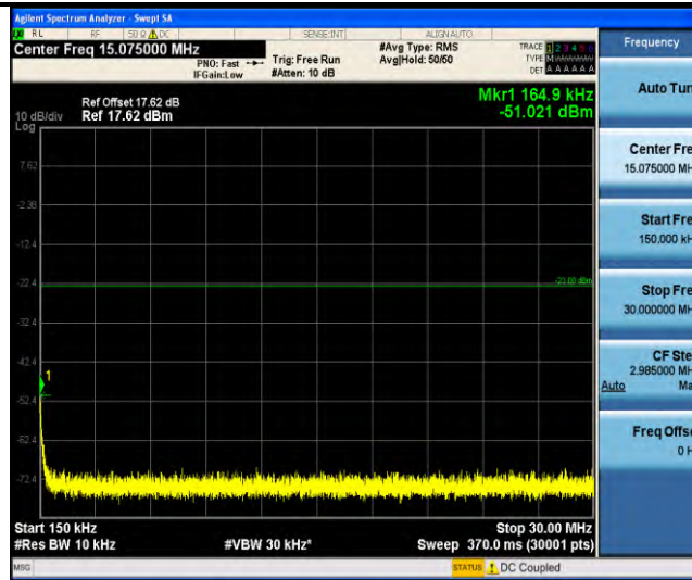
Band18-Stand-Alone-NaN-QPSK-23925-1 @ 47-3.75kHz-0.15-30-0.15~30MHz @ -51.02dBm--23-PASS
