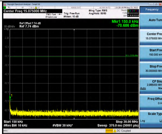
Band19-Stand-Alone-NaN-QPSK-24002-1 @0-3.75kHz-0.15-30-0.15~30MHz@-70.69dBm--23-PASS
