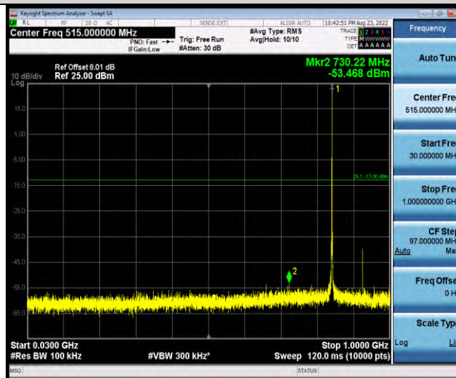
Band19-Stand-Alone-NaN-QPSK-24148-1 @ 47-3.75kHz-30-1000-30~1000MHz @ -53.47dBm--13-PASS
