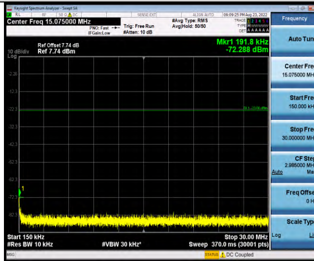
Band18-Stand-Alone-NaN-QPSK-23998-1 @ 47-3.75kHz-0.15-30-0.15~30MHz @ -72.29dBm--23-PASS
