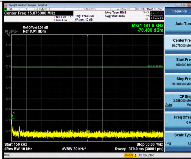
Band19-Stand-Alone-NaN-QPSK-24148-1 @ 47-3.75kHz-0.15-30-0.15~30MHz @ -70.48dBm--23-PASS
