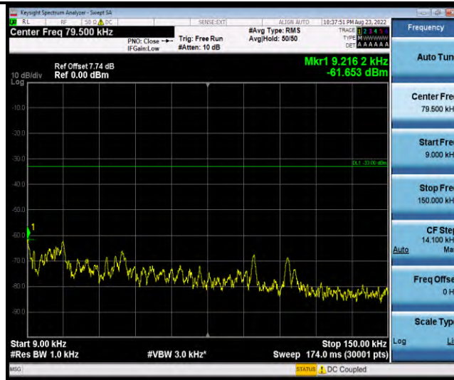
Band19-Stand-Alone-NaN-QPSK-24002-1 @0-3.75kHz-0.009-0.15-0.009~0.15MHz@-61.65dBm--33-PASS
