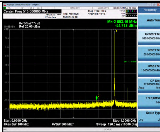
Band19-Stand-Alone-NaN-QPSK-24002-1 @0-3.75kHz-30-1000-30~1000MHz@-54.72dBm--13-PASS
