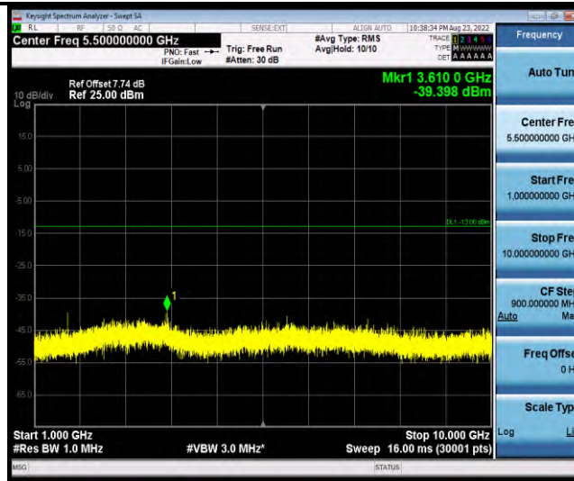
Band19-Stand-Alone-NaN-QPSK-24002-1 @ 0-3.75kHz-1000-10000-1000~10000MHz @ -39.4dBm--13-PASS
