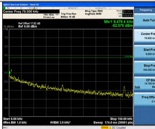
Band18-Stand-Alone-NaN-QPSK-23925-1 @47-3.75kHz-0.009-0.15-0.009~0.15MHz @-52.58dBm--33-PASS
