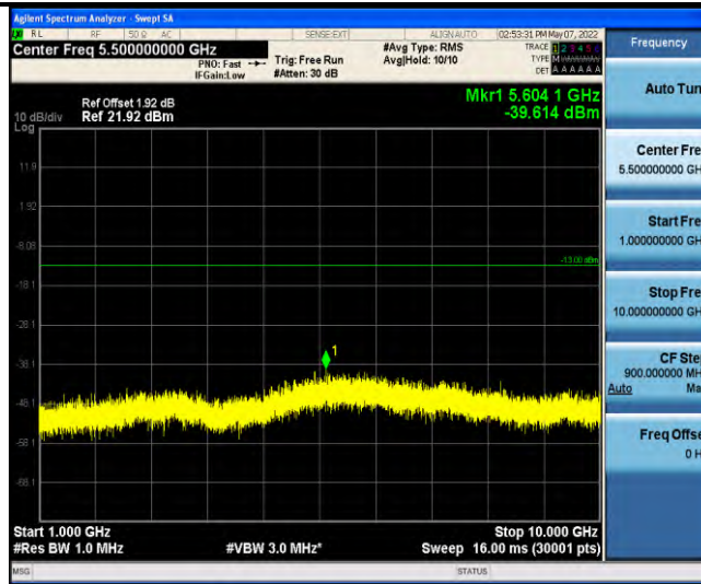
Band13-Stand-Alone-NaN-QPSK-23278-1 @0-3.75kHz-1000-10000-1000~1000MHz @ -39.61dBm--13-PASS
