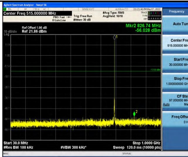
Band12-Stand-Alone-NaN-QPSK-23012-1 @47-3.75kHz-30-1000-30~1000MHz @-56.03dBm--13-PASS
