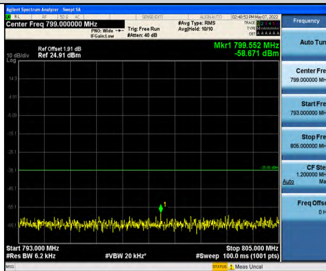
Band13-Stand-Alone-NaN-QPSK-23182-1 @ 47-3.75kHz-793-805-793~805MHz @ -58.67dBm--35-PASS
