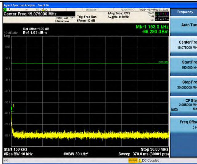
Band13-Stand-Alone-NaN-QPSK-23278-1 @ 47-3.75kHz-0.15-30-0.15~30MHz @ -66.29dBm--23-PASS
