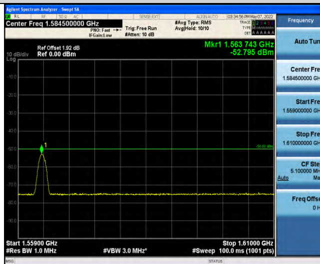
Band13-Stand-Alone-NaN-QPSK-23230-1 @0-3.75kHz-1559-1610-1559~1610MHz @ -52.8dBm--50-PASS
