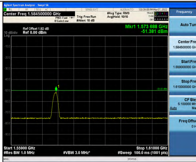
Band13-Stand-Alone-Na-N-BPSK-23278-1 @ 0-15kHz-1559-1610-1559~1610MHz @ -51.38dBm--50-PASS
