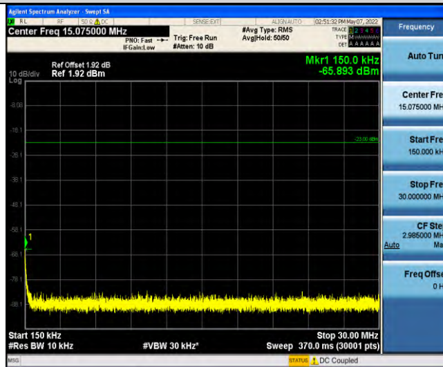
Band13-Stand-Alone-NaN-QPSK-23230-1 @ 47-3.75kHz-0.15-30-0.15~30MHz @ -65.89dBm--23-PASS
