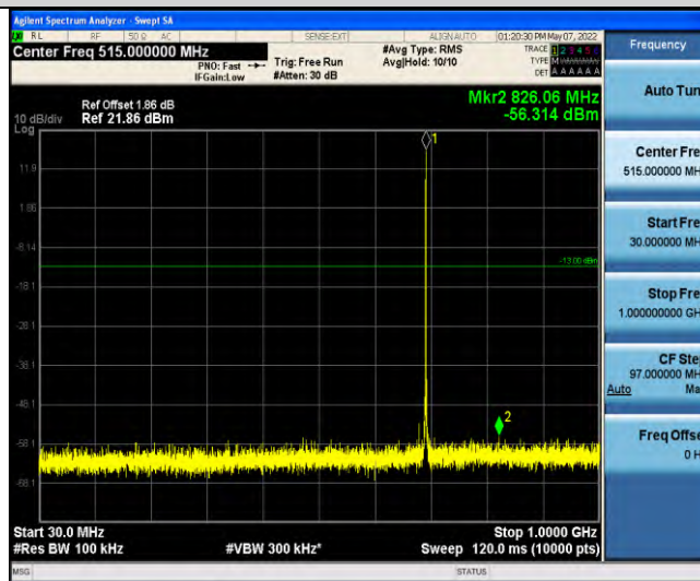
Band12-Stand-Alone-Na-N-QPSK-23012-1 @0-3.75kHz-30-1000-30~1000MHz@-56.31dBm--13-PASS
