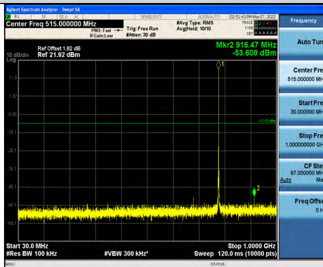
Band13-Stand-Alone-NaN-QPSK-23230-1 @ 47-3.75kHz-30-1000-30~1000MHz @ -53.61dBm--13-PASS
