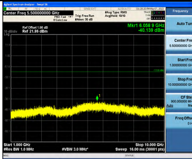
Band12-Stand-Alone-NaN-QPSK-23012-12@0-15kHz-1000-10000-1000~1000MHz@-40.14dBm--13-PASS
