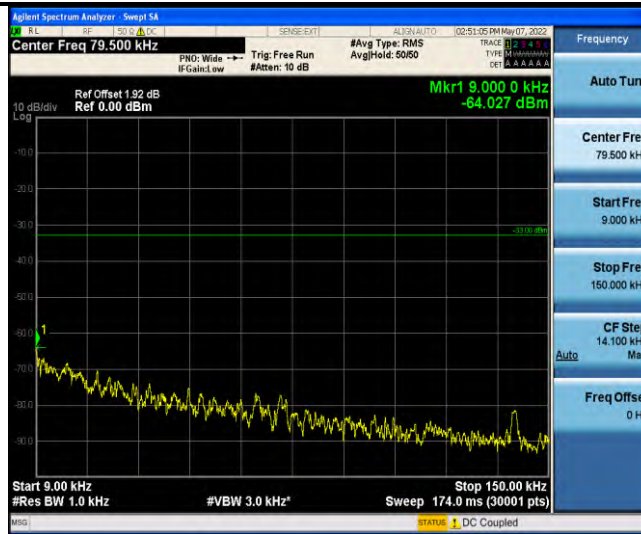
Band13-Stand-Alone-NaN-QPSK-23230-1 @ 47-3.75kHz-0.009-0.15-0.009~0.15MHz @ -64.03dBm--33-PASS
