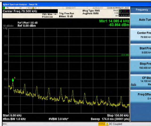
Band13-Stand-Alone-Na-N-BPSK-23278-1 @ 11-15kHz-0.009-0.15-0.009~0.15MHz @ -63.86dBm--33-PASS
