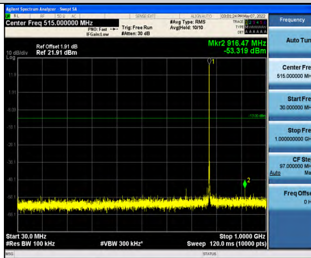
Band13-Stand-Alone-NaN-BPSK-23182-1@0-15kHz-30-1000-30~1000MHz@-53.32dBm--13-PASS
