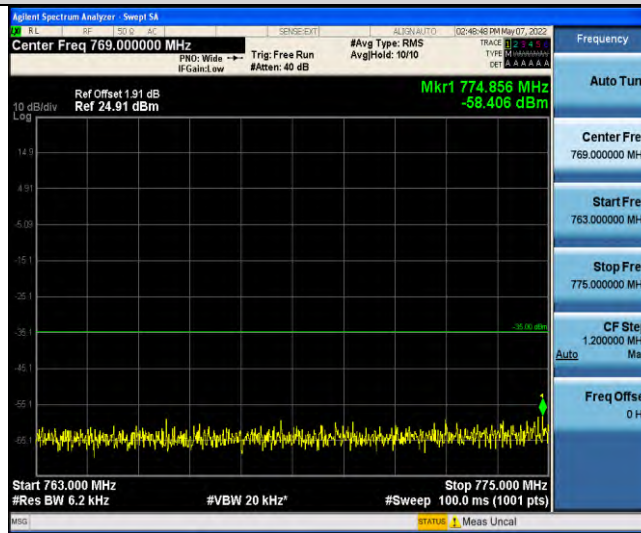
Band13-Stand-Alone-NaN-QPSK-23182-1 @ 47-3.75kHz-763-775-763~775MHz @ -58.41dBm--35-PASS
