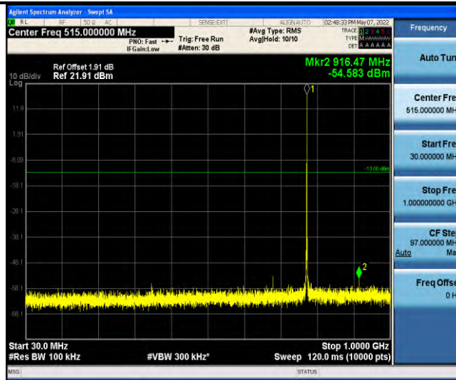
Band13-Stand-Alone-NaN-QPSK-23182-1 @ 47-3.75kHz-30-1000-30~1000MHz @ -54.58dBm--13-PASS
