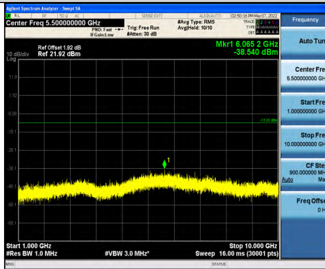
Band13-Stand-Alone-NaN-QPSK-23230-1 @0-3.75kHz-1000-10000-1000~10000MHz @ -38.54dBm--13-PASS
