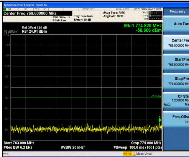
Band13-Stand-Alone-NaN-BPSK-23182-1 @ 0-15kHz-763-775-763~775MHz @ -58.61dBm--35-PASS
