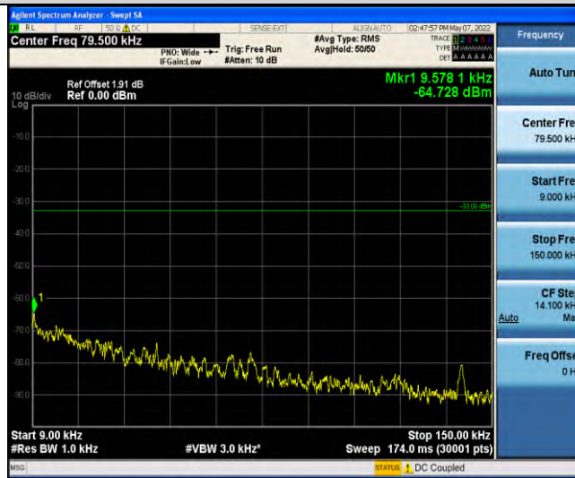
Band13-Stand-Alone-Na-N-QPSK-23182-1 @47-3.75kHz-0.009-0.15-0.009~0.15MHz@-64.73dBm--33-PASS
