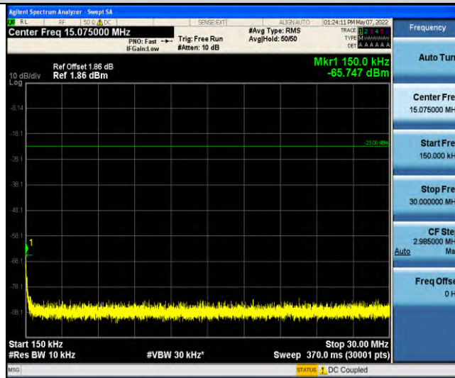
Band12-Stand-Alone-Na-N-QPSK-23095-1 @ 47-3.75kHz-0.15-30-0.15~30MHz @ -65.75dBm--23-PASS
