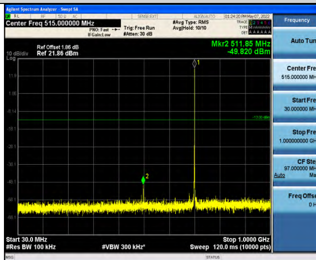
Band12-Stand-Alone-Na-N-QPSK-23095-1 @ 47-3.75kHz-30-1000-30~1000MHz @ -49.82dBm--13-PASS
