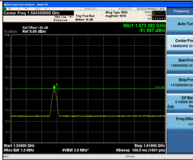
Band13-Stand-Alone-NaN-QPSK-23278-1 @0-3.75kHz-1559-1610-1559~1610MHz @ -51.6dBm--50-PASS
