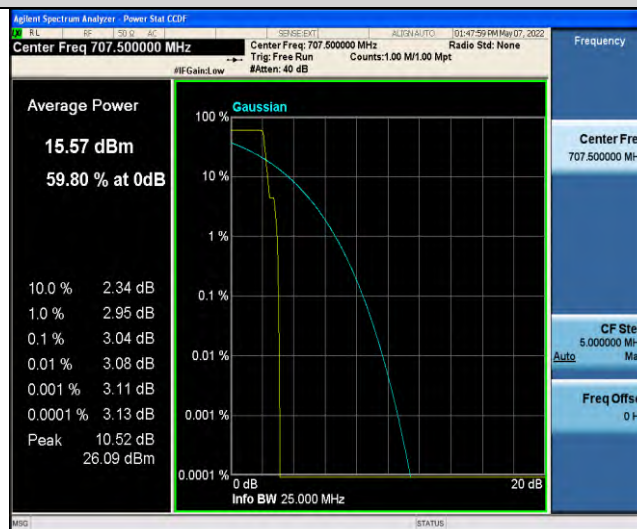
Band12-Stand-Alone-NaN-QPSK-23095-1 @0-3.75kHz-3.04-<=13-PASS
