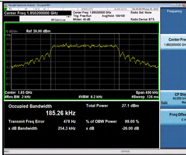
Band2-Stand-Alone-NaN-BPSK-18602-12 @0-15kHz-0.2543-PASS
