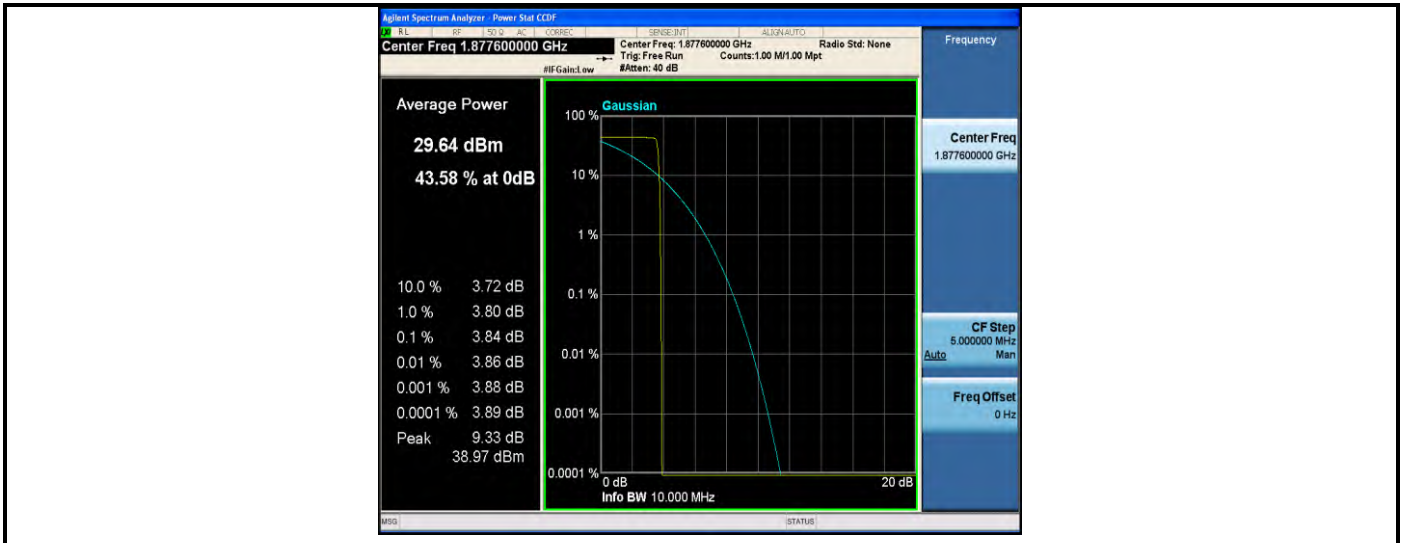
Band2-Stand-Alone-NaN-BPSK-18876-1 @0-3.75kHz-3.84-<=13-PASS
