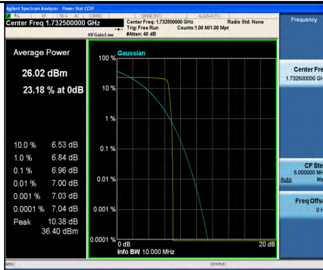
Band4-Stand-Alone-NaN-BPSK-20175-1 @ 11-15kHz-6.96-<=13-PASS
