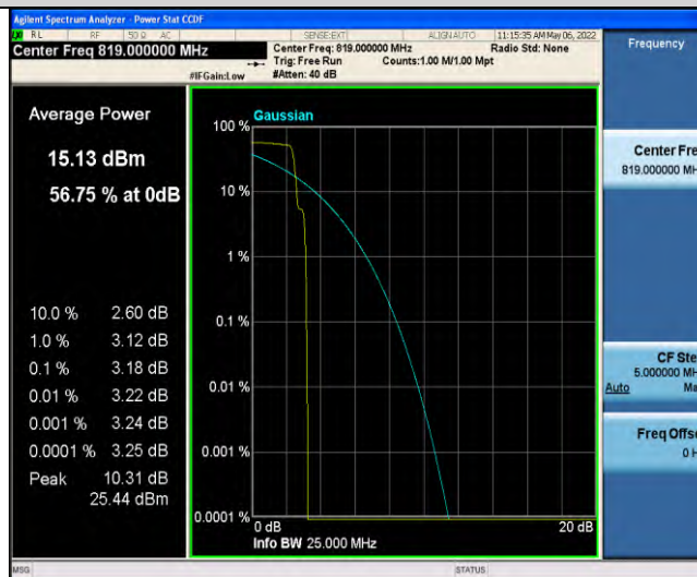
Band26-Stand-Alone-NaN-BPSK-26740-1 @ 11-15kHz-3.18-<=13-PASS
