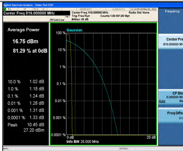
Band26-Stand-Alone-NaN-QPSK-26740-1 @47-3.75kHz-1.24-<=13-PASS
