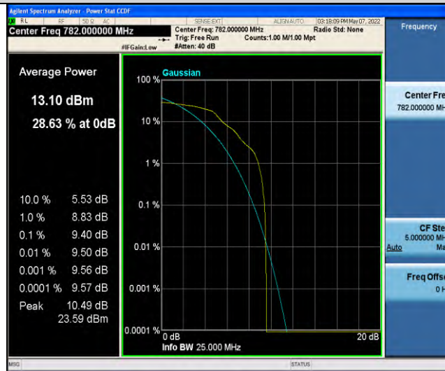
Band13-Stand-Alone-NaN-QPSK-23230-3 @ 3-15kHz-9.4-<=13-PASS
