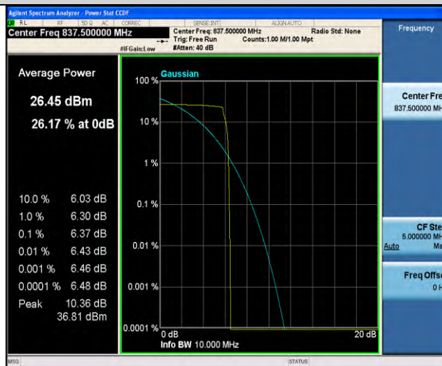
Band19-Stand-Alone-NaN-BPSK-24075-1 @0-15kHz-6.37-<=13-PASS
