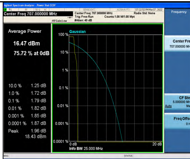
Band85-Stand-Alone-NaN-BPSK-134092-1 @ 47-3.75kHz-1.79-<=13-PASS
