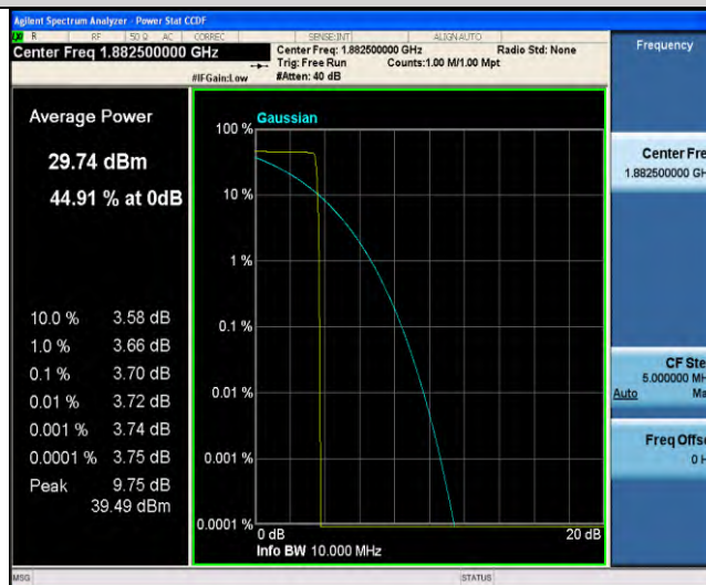
Band25-Stand-Alone-NaN-BPSK-26365-1 @ 0-3.75kHz-3.7-<=13-PASS
