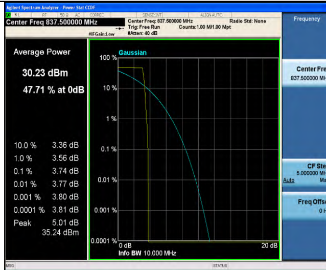
Band19-Stand-Alone-NaN-QPSK-24075-1 @47-3.75kHz-3.74-<=13-PASS
