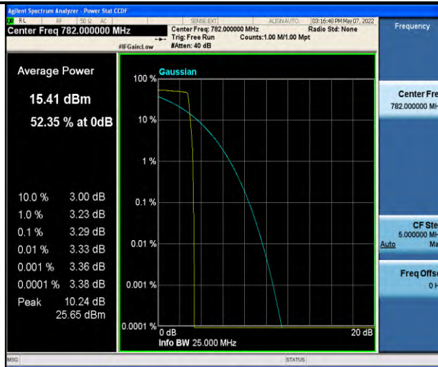
Band13-Stand-Alone-NaN-BPSK-23230-1 @ 11-15kHz-3.29-<=13-PASS
