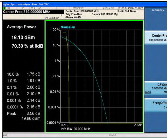
Band26-Stand-Alone-NaN-QPSK-26740-1 @0-3.75kHz-2.06-<=13-PASS
