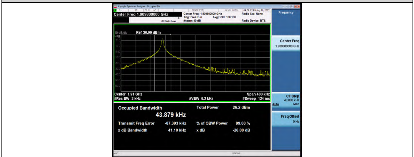
Band2-Stand-Alone-NaN-BPSK-19198-1 @ 0-3.75kHz-0.0411-PASS
