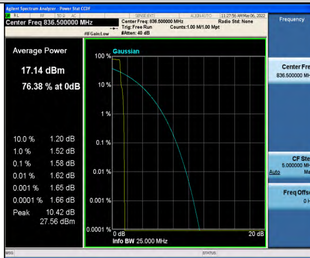
Band26-Stand-Alone-NaN-BPSK-26915-1 @0-3.75kHz-1.58-<=13-PASS
