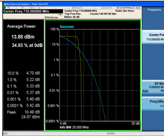
Band17-Stand-Alone-NaN-QPSK-23790-1 @11-15kHz-5.33-<=13-PASS
