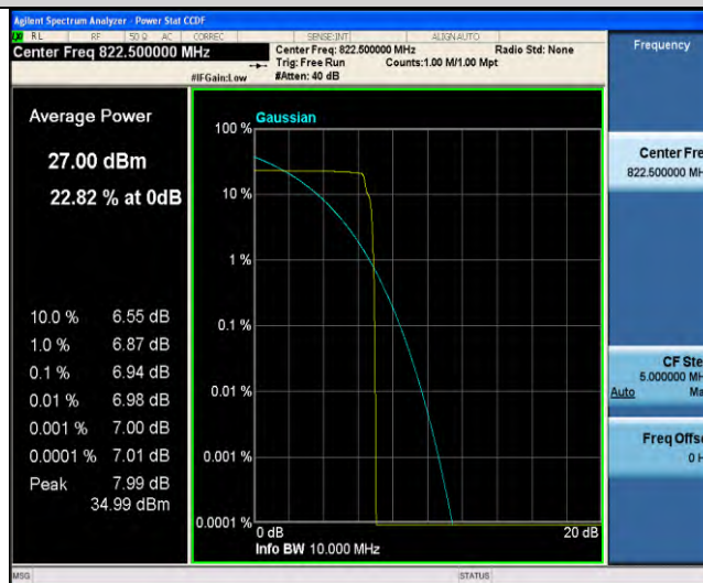
Band18-Stand-Alone-NaN-QPSK-23925-1 @11-15kHz-6.94-<=13-PASS
