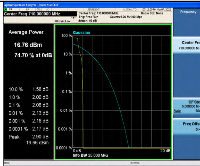
Band17-Stand-Alone-NaN-QPSK-23790-1 @0-3.75kHz-2.08-<=13-PASS
