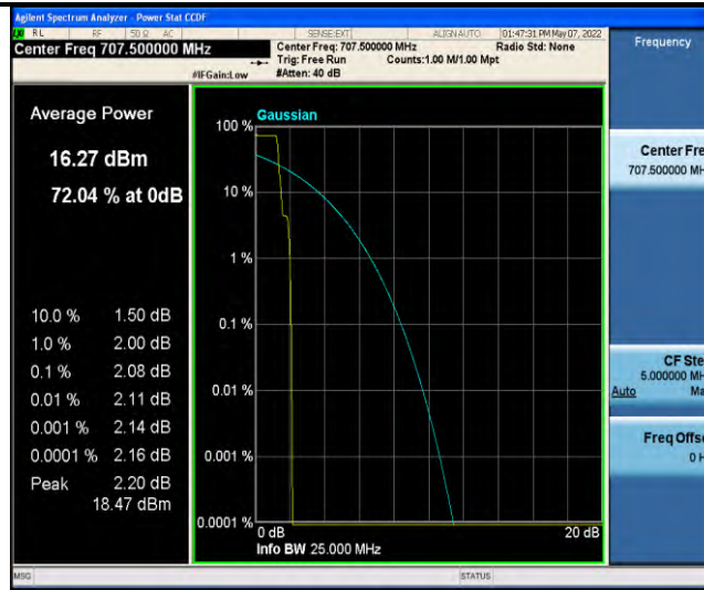
Band12-Stand-Alone-NaN-BPSK-23095-1 @0-3.75kHz-2.08-<=13-PASS
