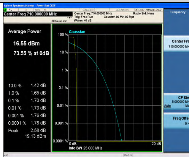
Band17-Stand-Alone-NaN-BPSK-23790-1 @ 0-3.75kHz-1.7-<=13-PASS
