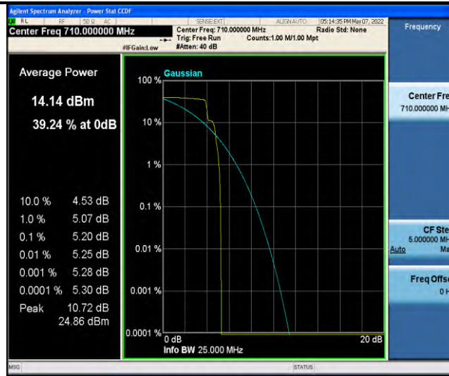
Band17-Stand-Alone-NaN-BPSK-23790-1 @ 0-15kHz-5.2-<=13-PASS
