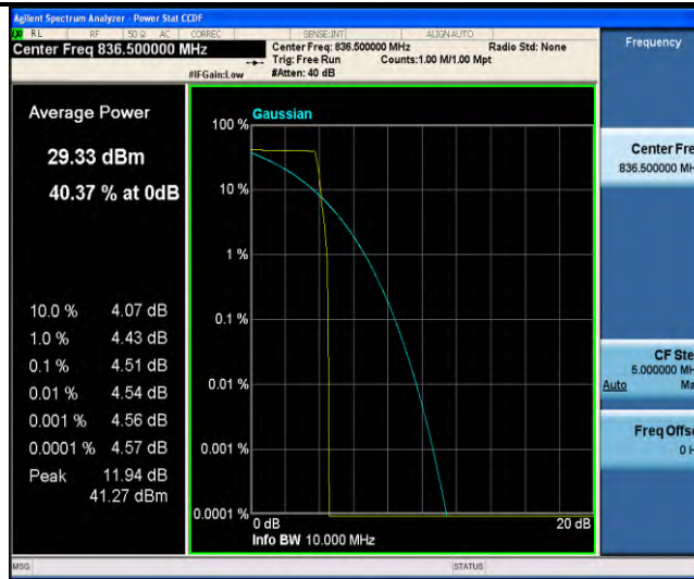
Band5-Stand-Alone-NaN-BPSK-20525-1 @47-3.75kHz-4.51-<=13-PASS
