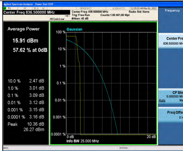
Band26-Stand-Alone-NaN-QPSK-26915-1 @47-3.75kHz-3.09-<=13-PASS
