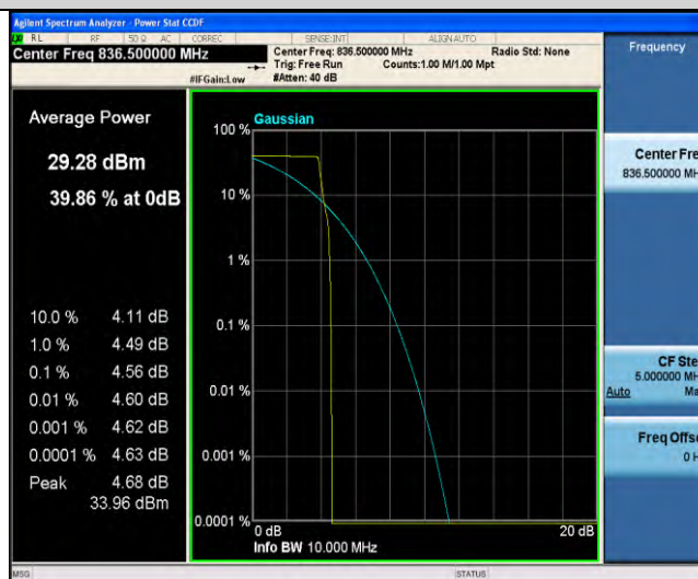
Band5-Stand-Alone-NaN-BPSK-20525-1 @ 0-3.75kHz-4.56-<=13-PASS
