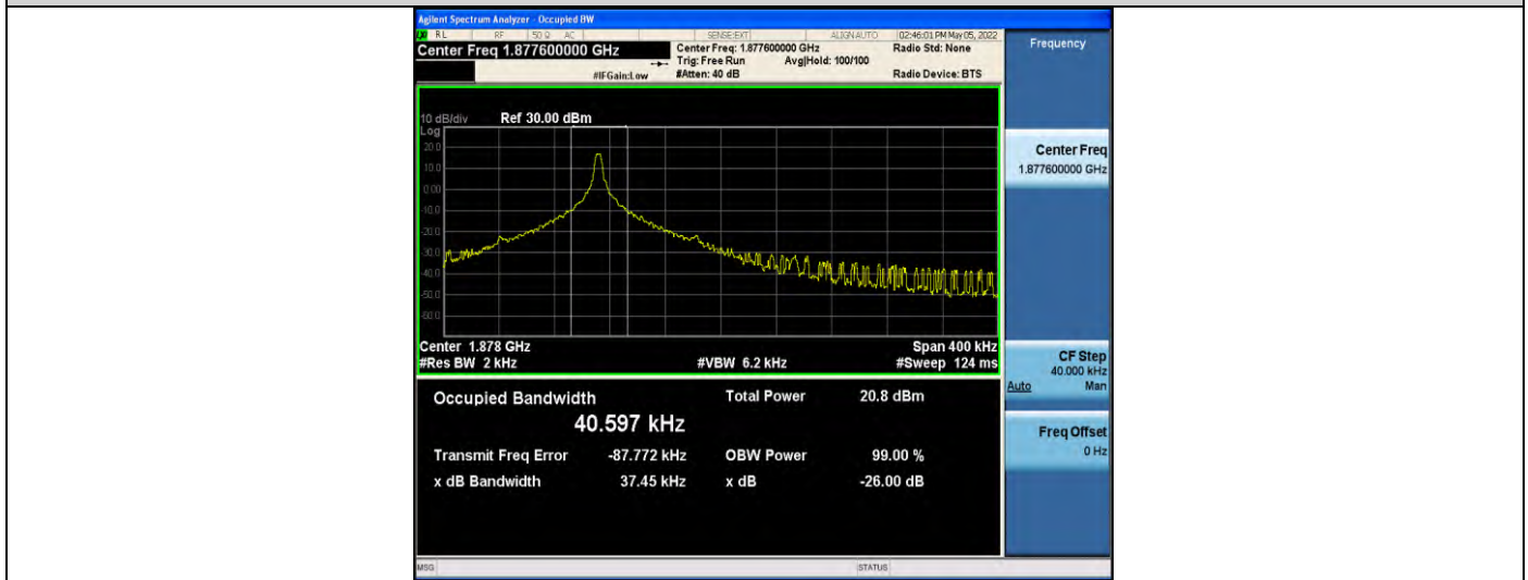
Band2-Stand-Alone-NaN-BPSK-18876-1 @ 0-3.75kHz-0.0374-PASS
