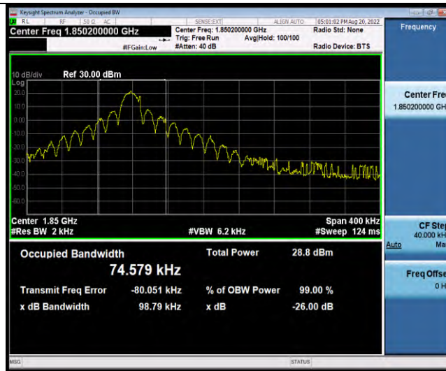
Band2-Stand-Alone-NaN-BPSK-18602-1 @0-15kHz-0.0988-PASS
