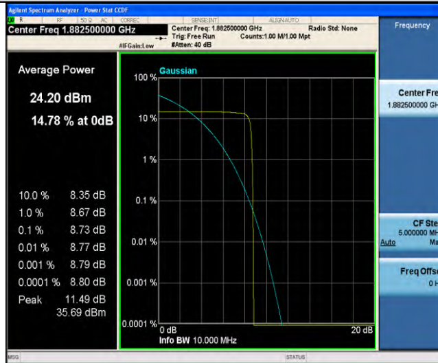
Band25-Stand-Alone-NaN-BPSK-26365-1 @ 11-15kHz-8.73-<=13-PASS
