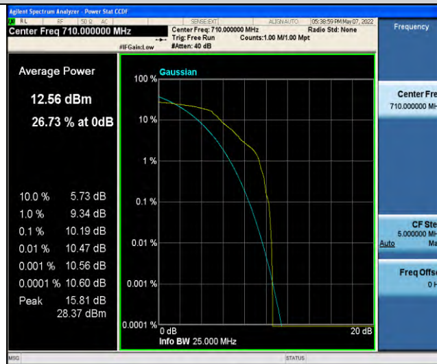
Band17-Stand-Alone-NaN-BPSK-23790-3 @ 3-15kHz-10.19-<=13-PASS
