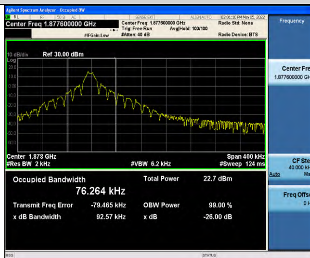
Band2-Stand-Alone-NaN-BPSK-18876-1 @0-15kHz-0.0926-PASS
