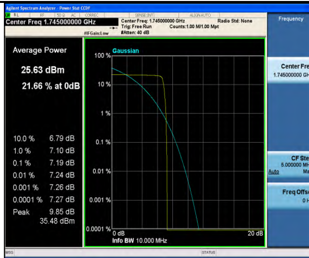
Band66-Stand-Alone-NaN-QPSK-132322-1 @ 11-15kHz-7.19-<=13-PASS
