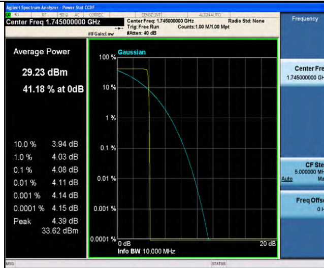
Band66-Stand-Alone-NaN-QPSK-132322-1 @47-3.75kHz-4.08-<=13-PASS
