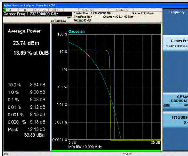
Band4-Stand-Alone-NaN-QPSK-20175-1 @ 0-15kHz-9.08-<=13-PASS
