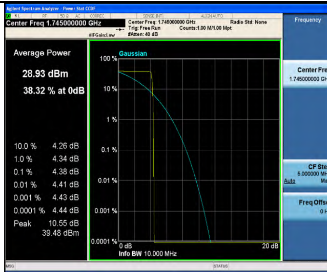
Band66-Stand-Alone-NaN-QPSK-132322-1 @0-3.75kHz-4.38-<=13-PASS
