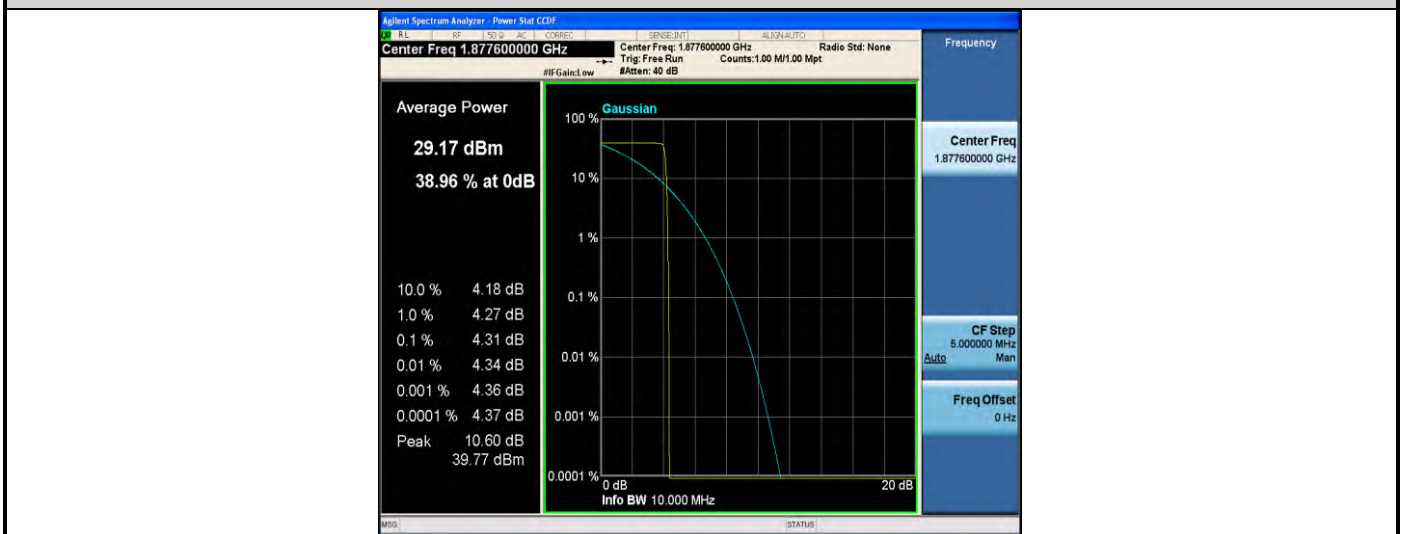
Band2-Stand-Alone-NaN-QPSK-18876-1 @0-3.75kHz-4.31-<=13-PASS
