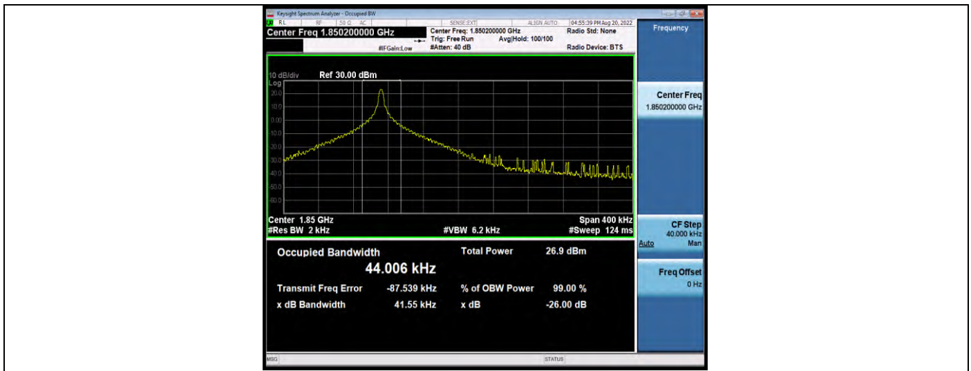
Band2-Stand-Alone-NaN-BPSK-18602-1 @ 0-3.75kHz-0.0415-PASS
