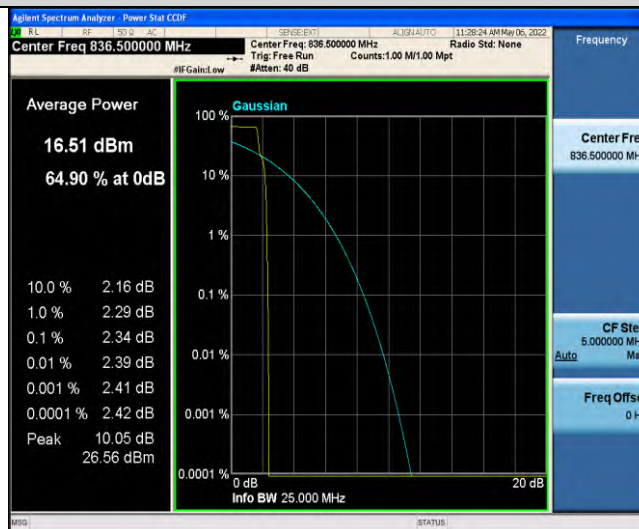
Band26-Stand-Alone-NaN-QPSK-26915-1 @0-3.75kHz-2.34-<=13-PASS
