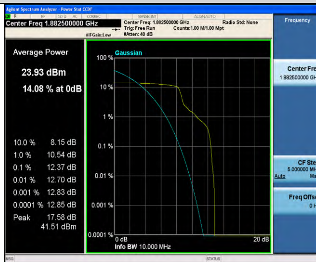
Band25-Stand-Alone-NaN-BPSK-26365-3 @ 3-15kHz-12.37-<=13-PASS
