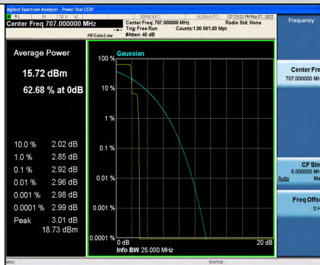
Band85-Stand-Alone-NaN-QPSK-134092-1 @ 47-3.75kHz-2.92-<=13-PASS
