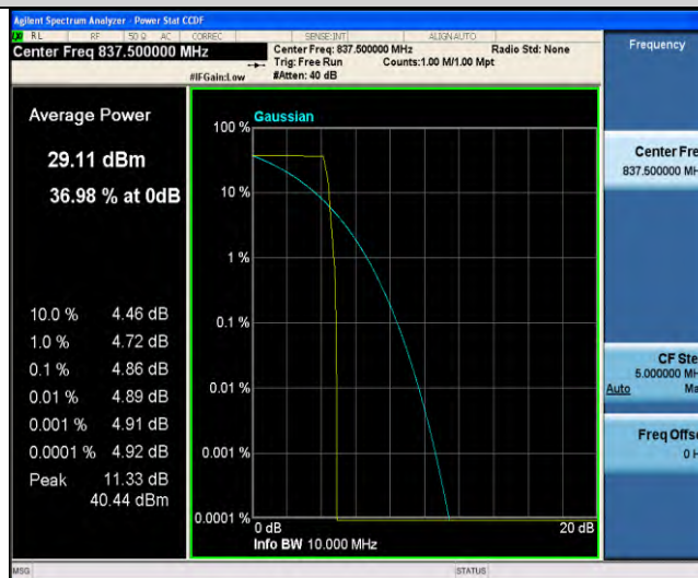
Band19-Stand-Alone-NaN-BPSK-24075-1@47-3.75kHz-4.86-<=13-PASS
