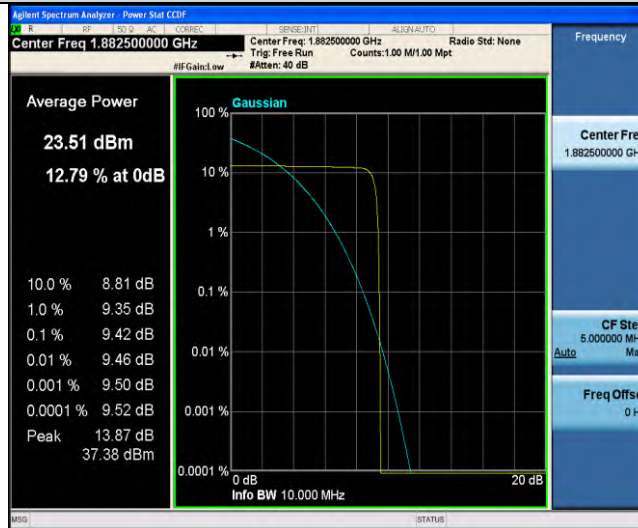
Band25-Stand-Alone-NaN-QPSK-26365-1 @ 11-15kHz-9.42-<=13-PASS
