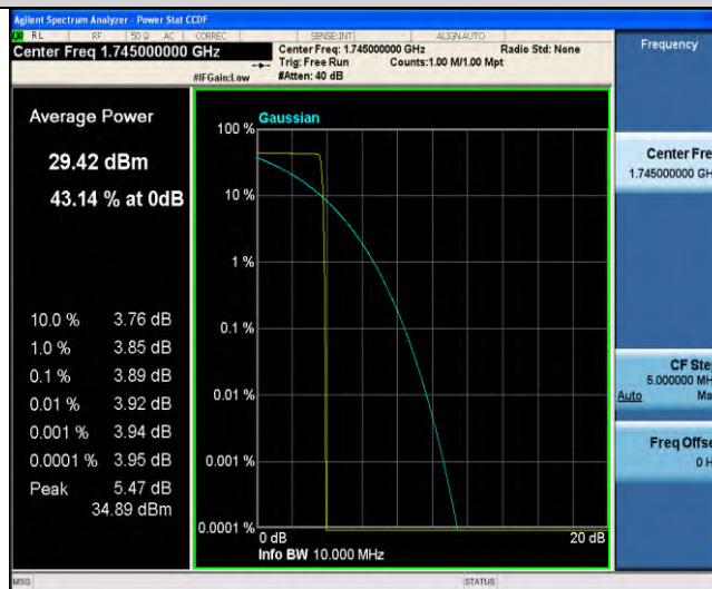
Band66-Stand-Alone-NaN-BPSK-132322-1@47-3.75kHz-3.89-<=13-PASS
