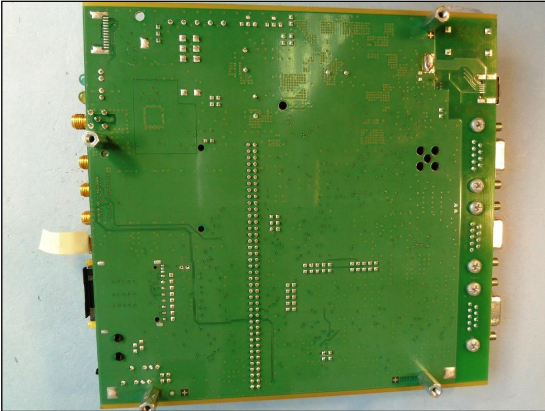
Photo 7: bottom view of the development board
