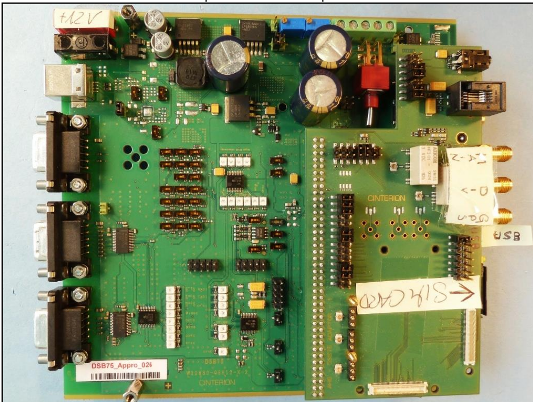
Photo 6: top view of the development board
