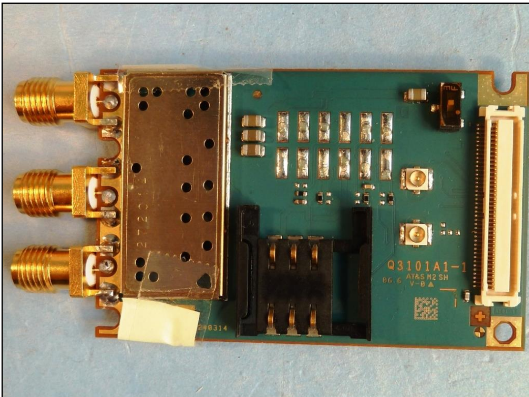
Photo 2: bottom view of the EUT
