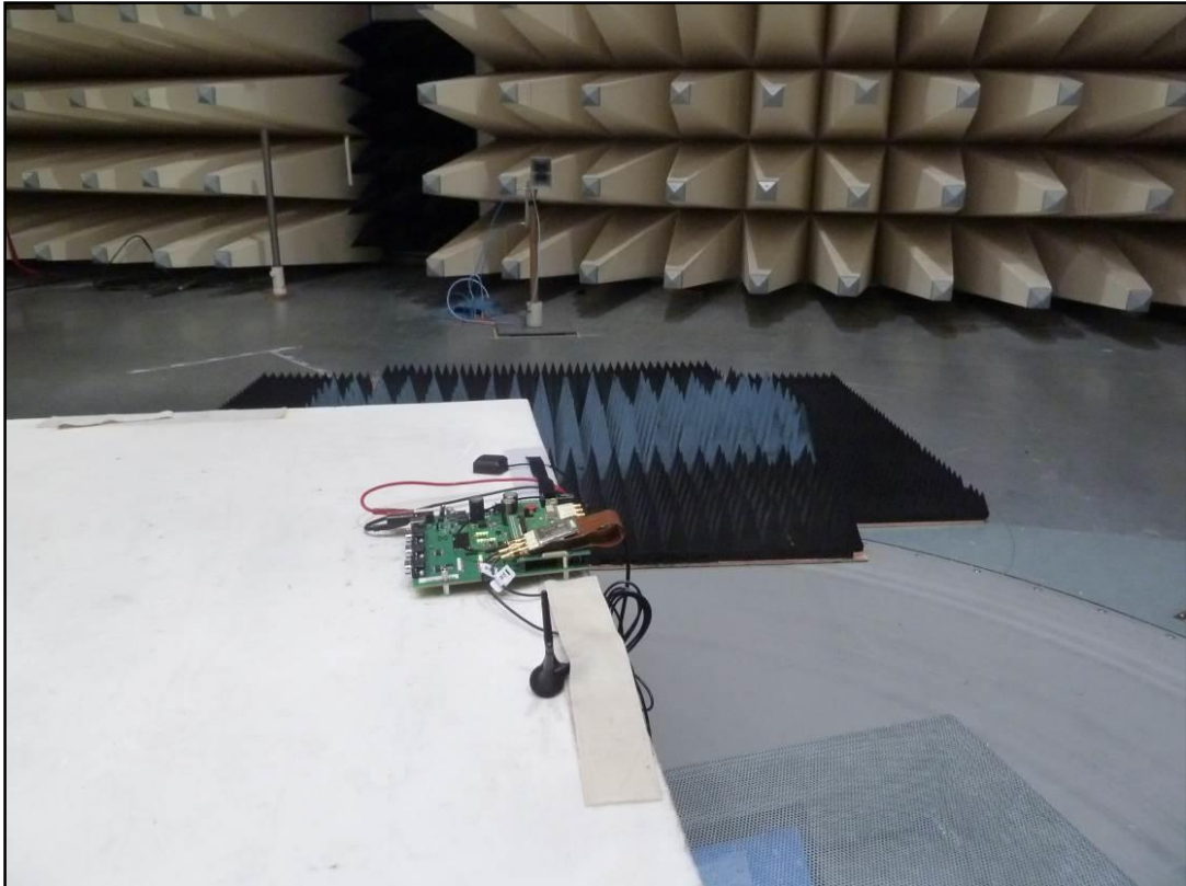
Photo 3: setup of radiated emission > 1 GHz
