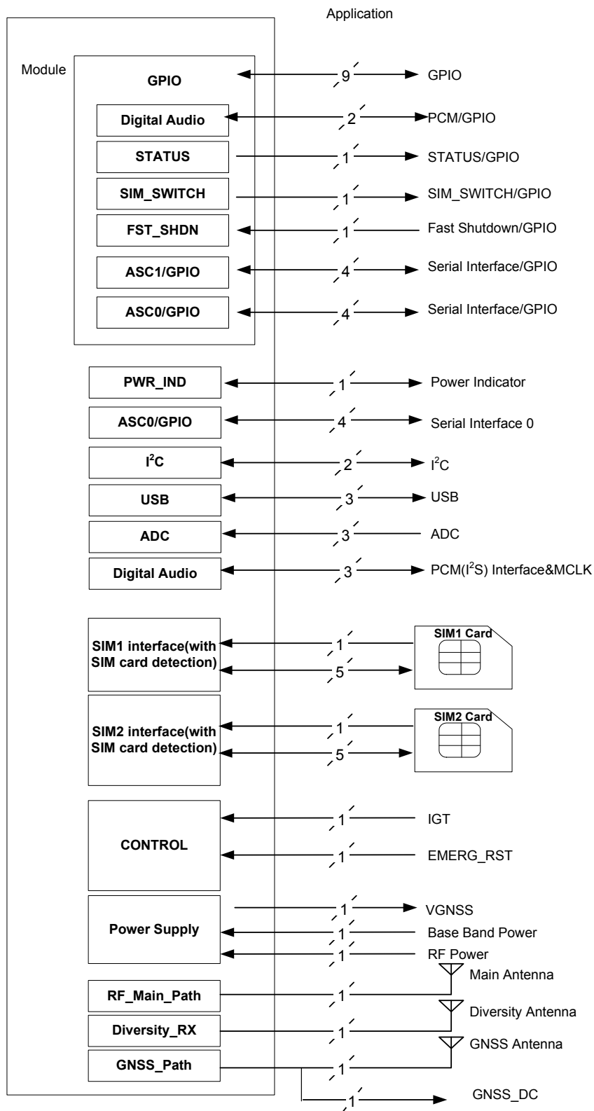
Figure 1: PLS63-X system overview
