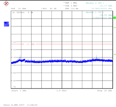
Channel 251: 1GHz~10GHz
