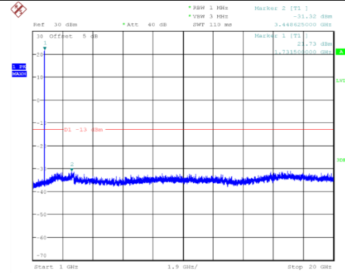
Channel 1450: 1GHz~20GHz
