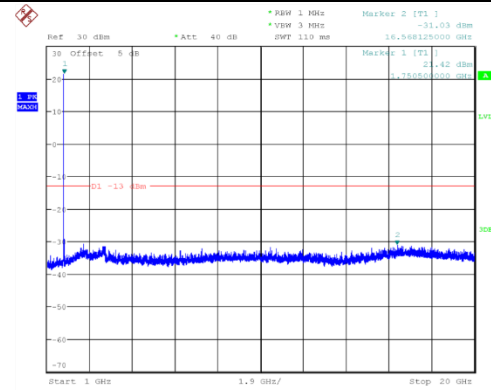
Channel 1512: 1GHz~20GHz
