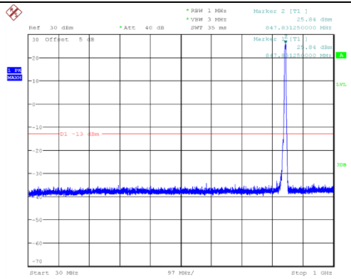
Channel 4232: 30MHz~1GHz
