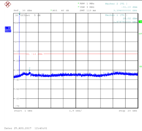
Channel 661: 1GHz~20GHz
