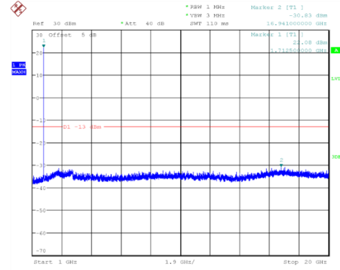
Channel 1312: 1GHz~20GHz
