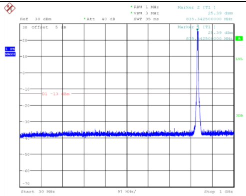
Channel 4175: 30MHz~1GHz
