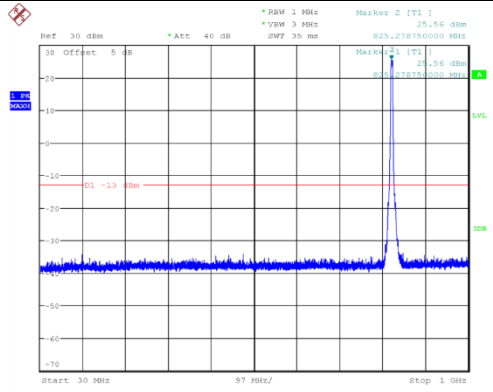
Channel 4133: 30MHz~1GHz
