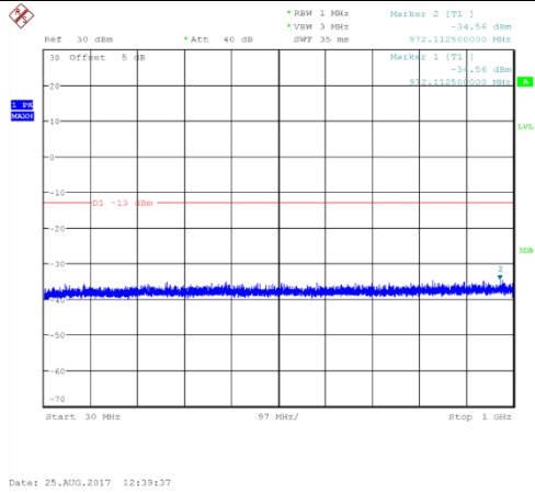
Channel 661: 30MHz~1GHz
