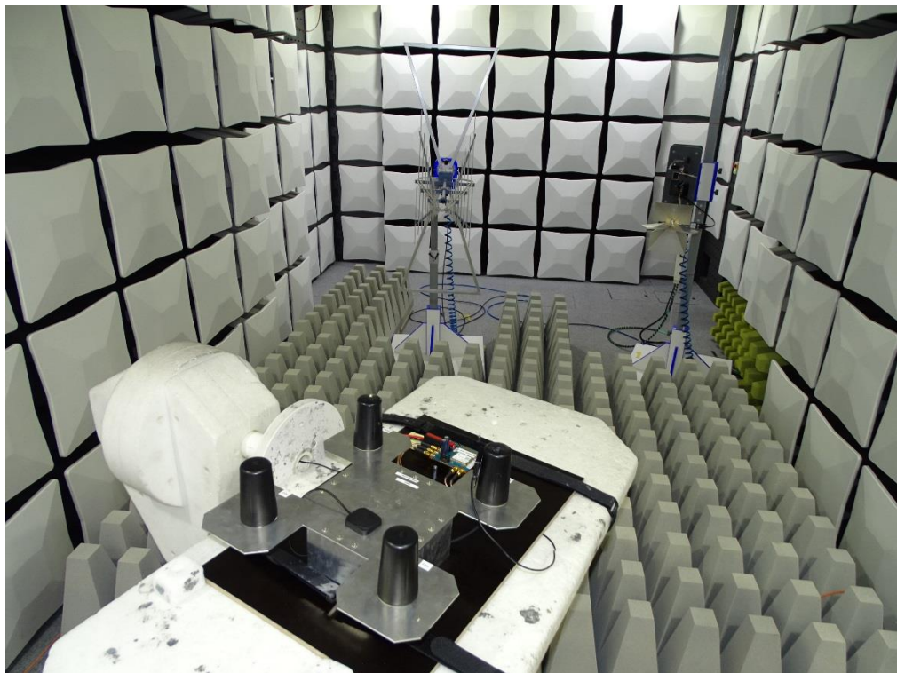
Photo 2: Test setup for radiated measurements above 1 GHz
