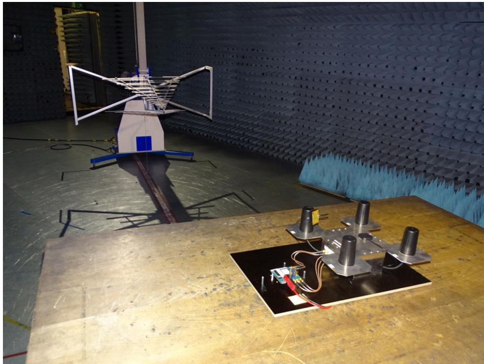
Photo 1: Test setup for radiated measurements below 1 GHz
