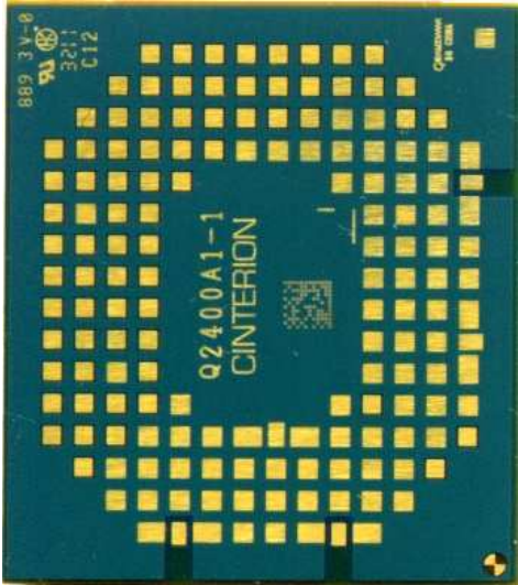
PHS8-US Bottom Side
