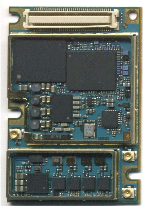
PH8 Top side
