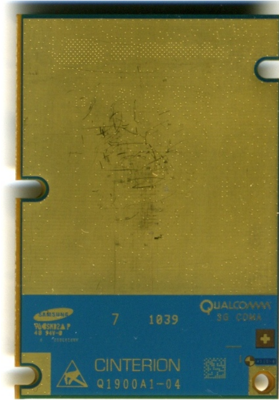
PH8 Bottom Side
