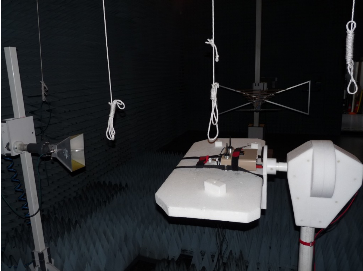
Photo 1: Setup for radiated tests, spurious emissions acc. to FCC Part 22, 24, 27
