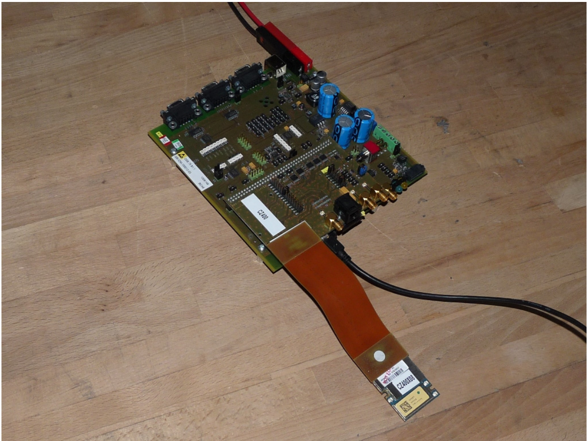
Photo 4: OUT setup (OUT and auxiliary equipment)
