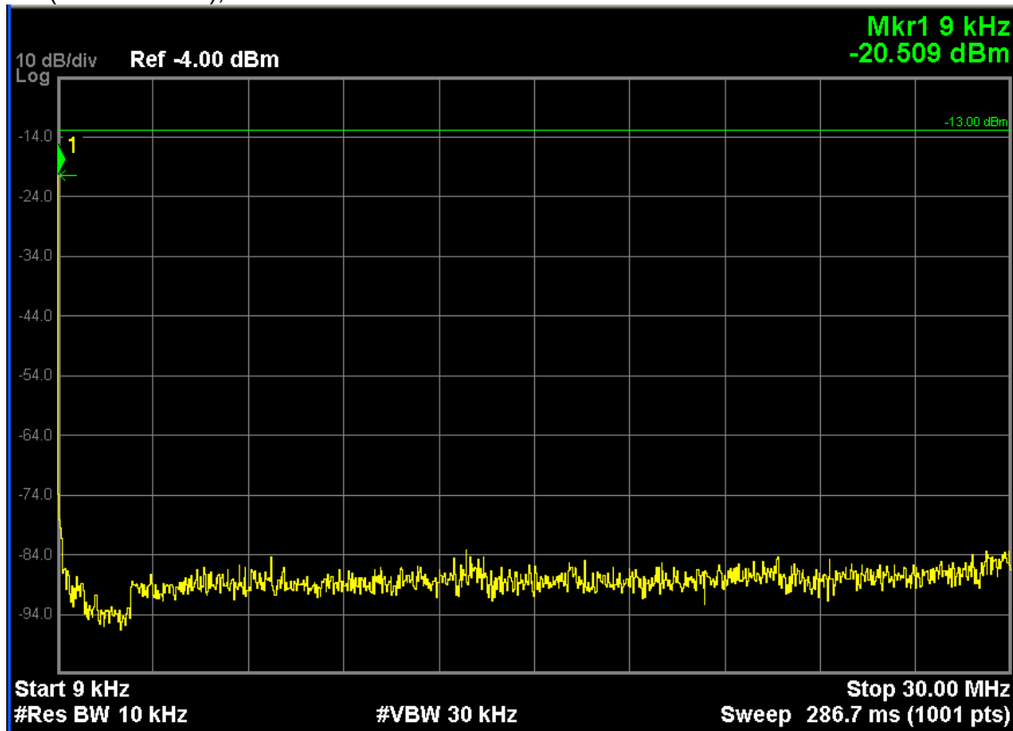
GSM850 (EDGE 8 Link), Channel 189
