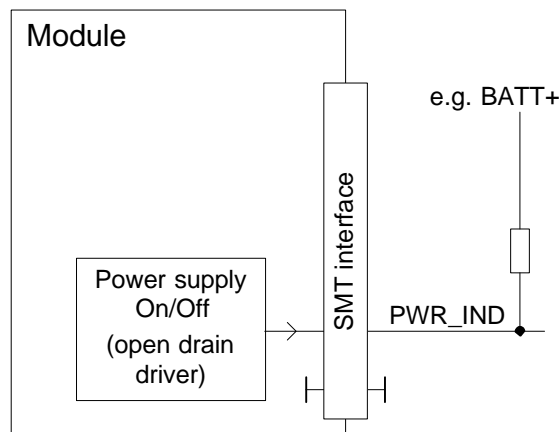
Figure 21: PWR_IND signal
