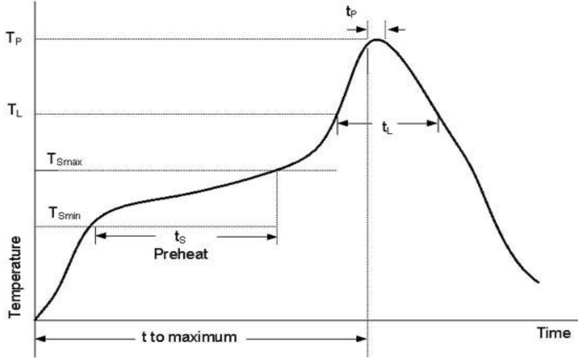
Figure 40: Reflow Profile
